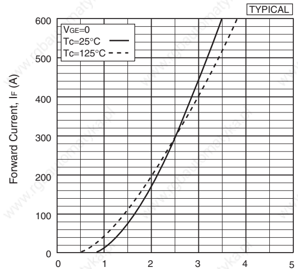
Forward voltage of free-wheeling diode
