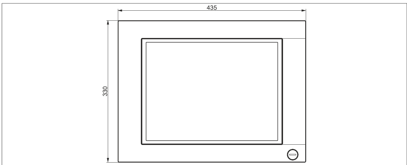
Figure 69: 5AP1120.1505-000 - Dimensions
