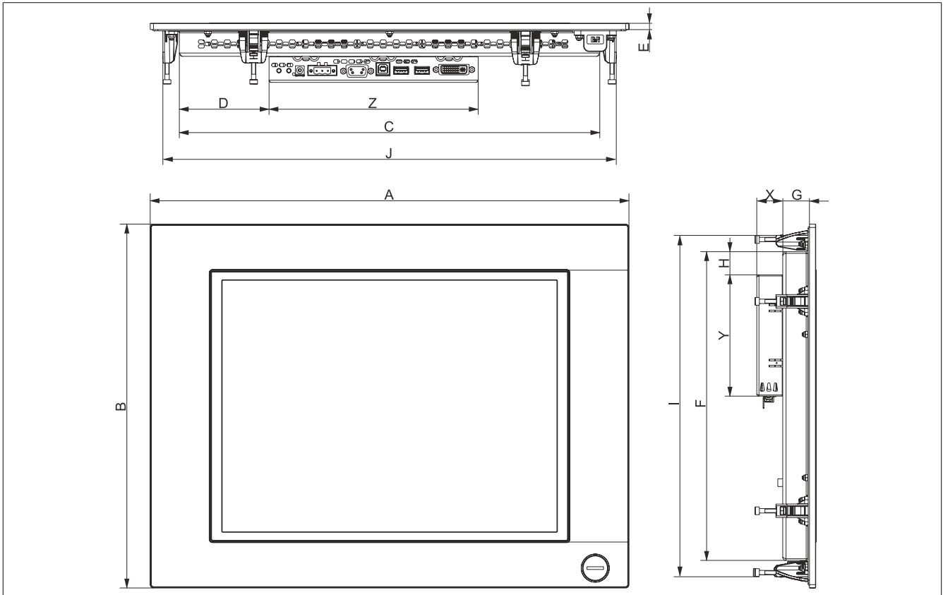
Figure 3: Automation Panel 1000 with clamping blocks - Dimensions
