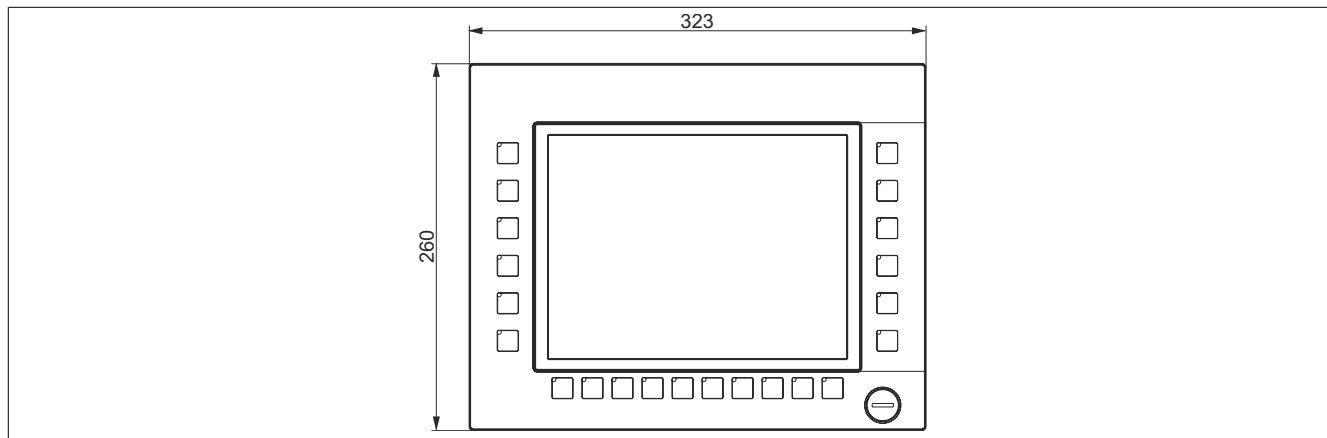
Figure 57: 5AP1180.1043-000 - Dimensions
