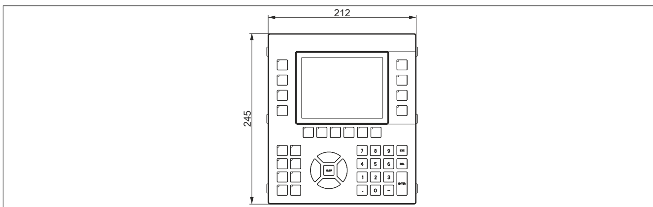
Figure 44: 5AP1151.0573-000 - Dimensions
