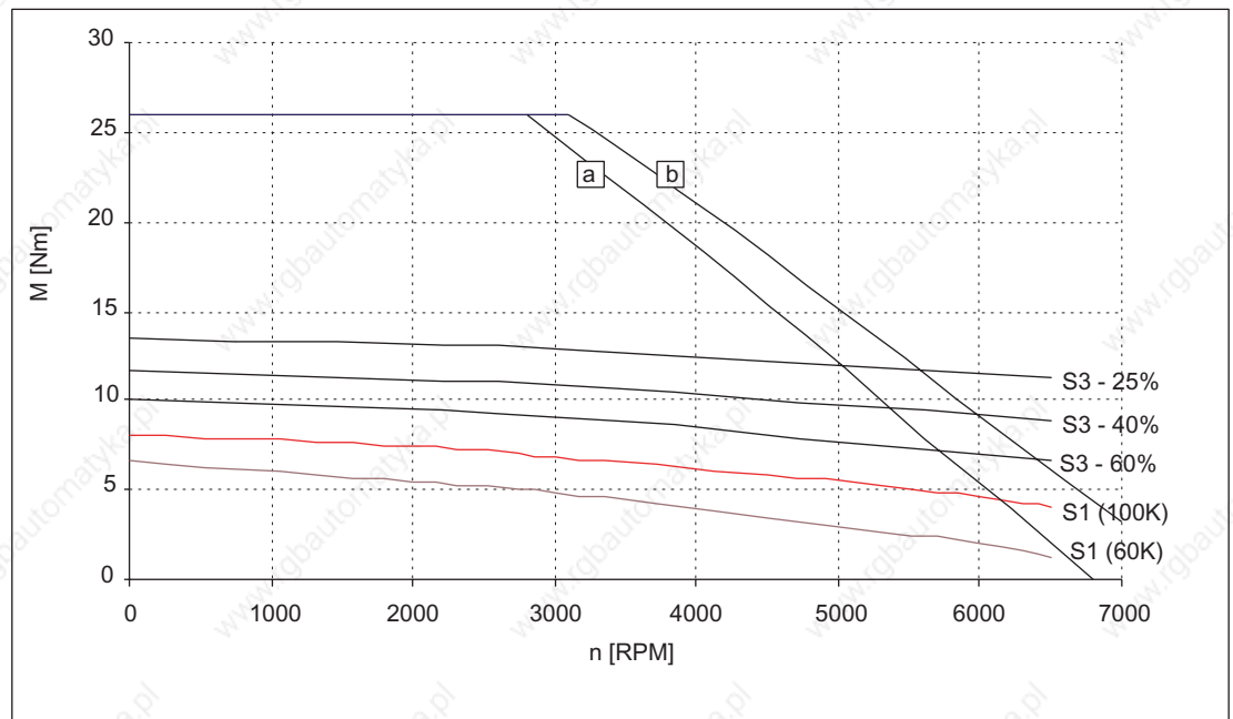
Figure 3-23 Speed-torque diagram 1FT6081-8AH7
