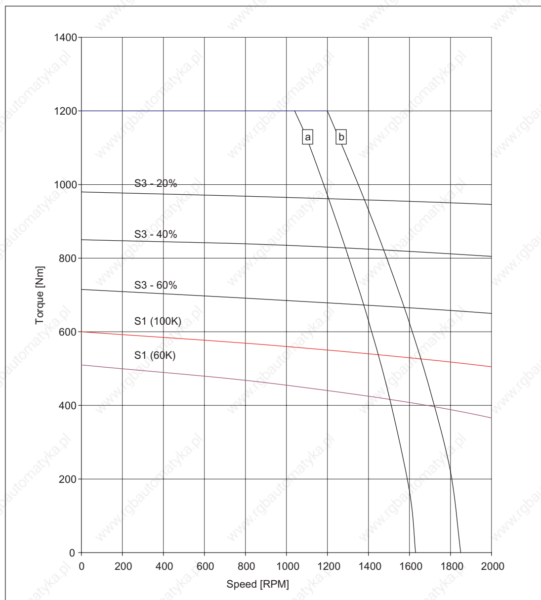
Figure 3-77 Speed-torque diagram 1FT6168-8SB7
