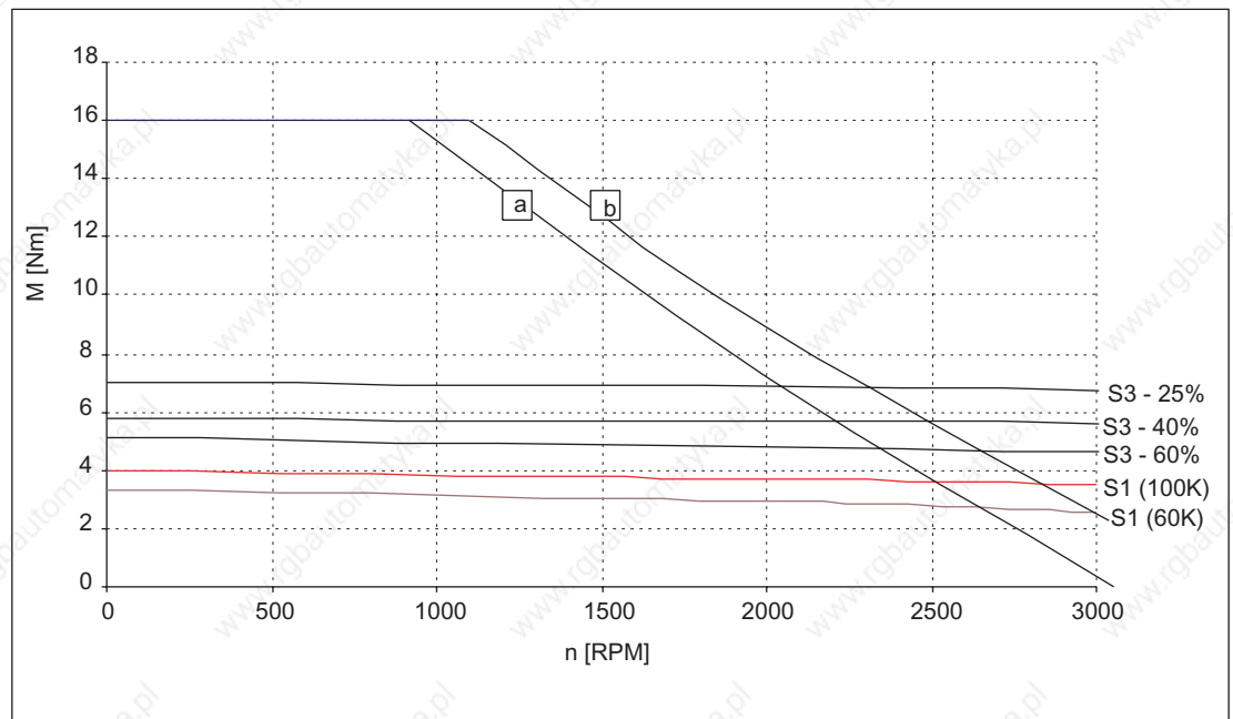
Figure 3-9 Speed-torque diagram 1FT6061-6AC7□
