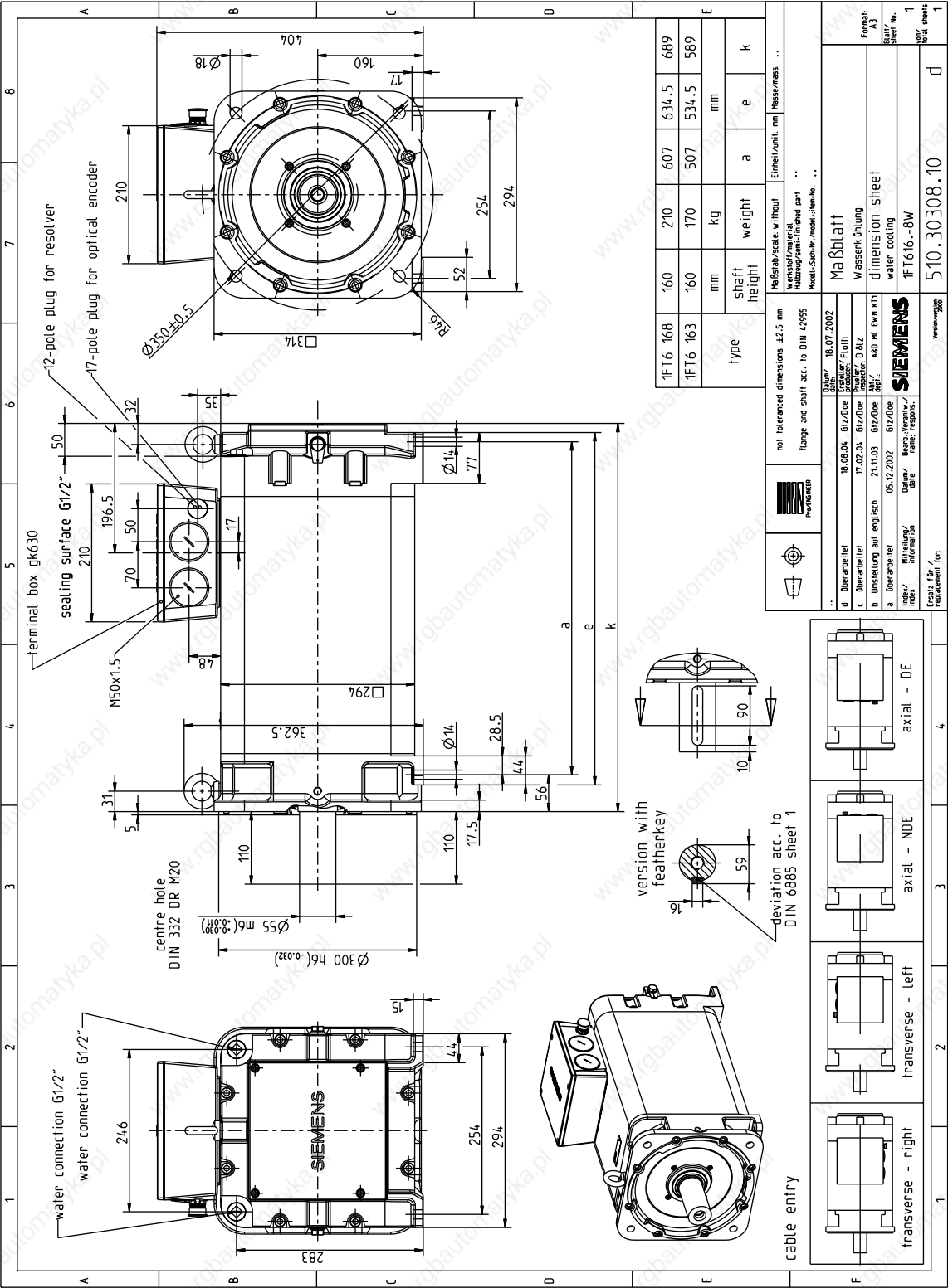
Figure 5-41 1FT616x-8Wx76-5xxx
