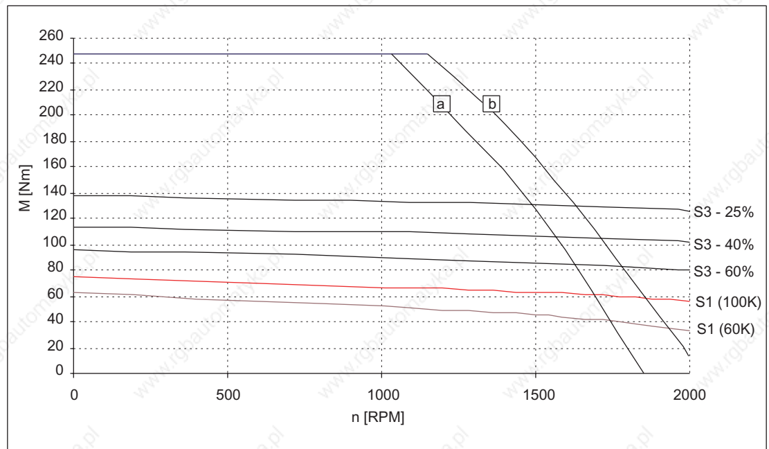
Figure 3-46 Speed-torque diagram 1FT6132-6AB71
