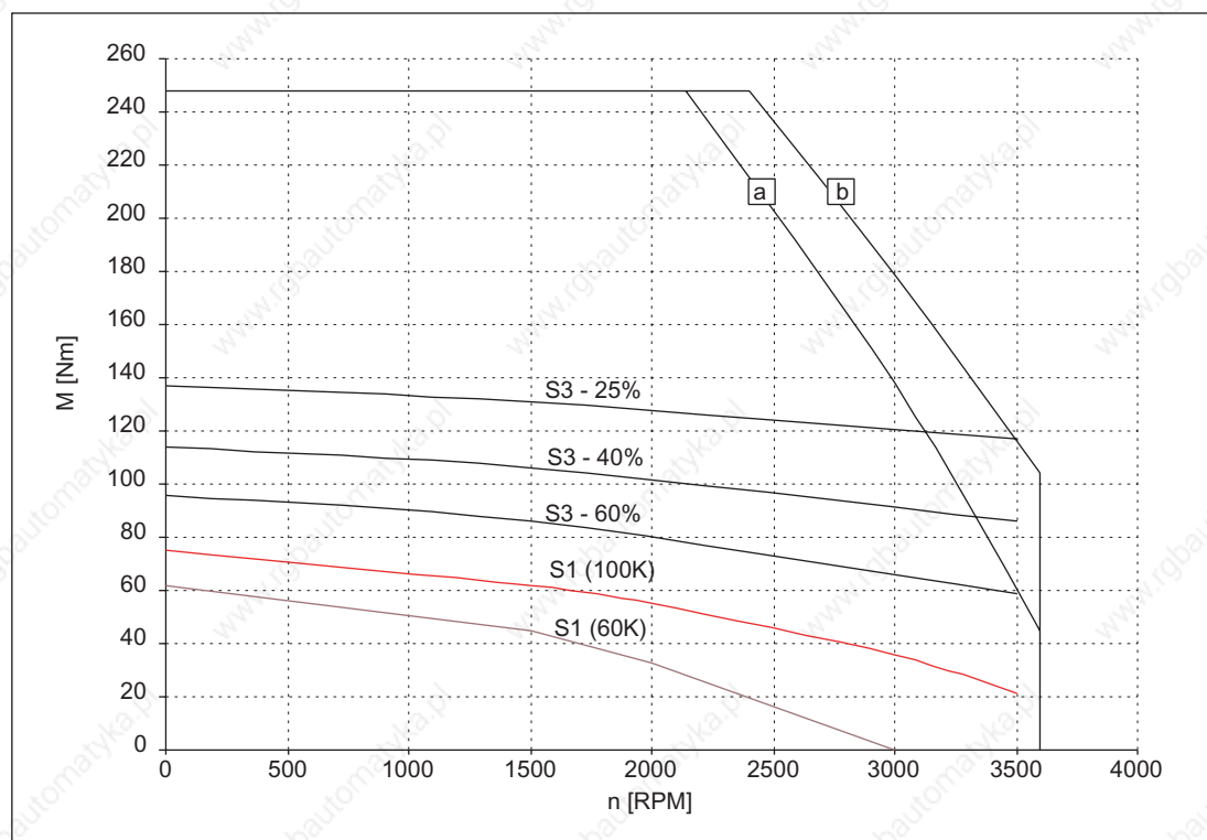
Figure 3-48 Speed-torque diagram 1FT6132-6AF71
