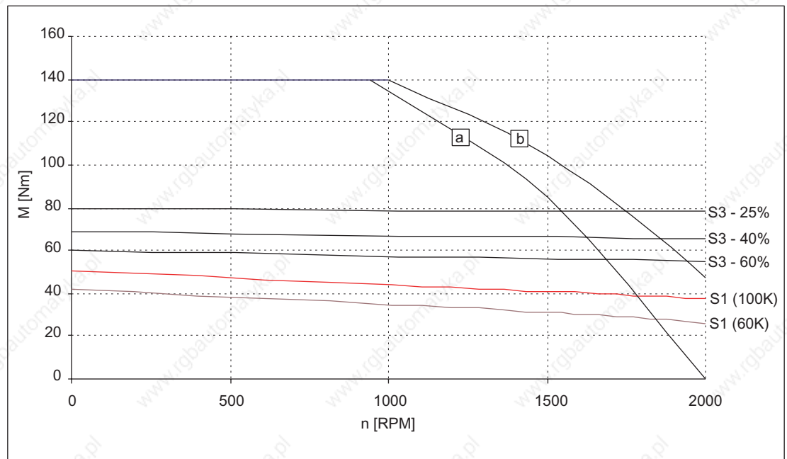
Figure 3-40 Speed-torque diagram 1FT6105-8AB7□
