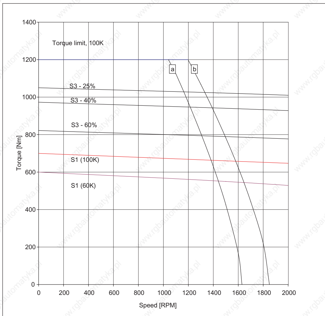
Figure 3-105 Speed-torque diagram 1FT6168-8WB7
