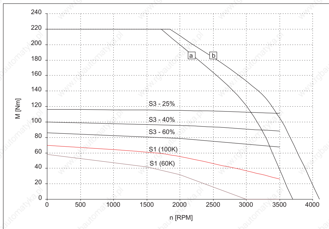
Figure 3-45 Speed-torque diagram 1FT6108-8AF7□
