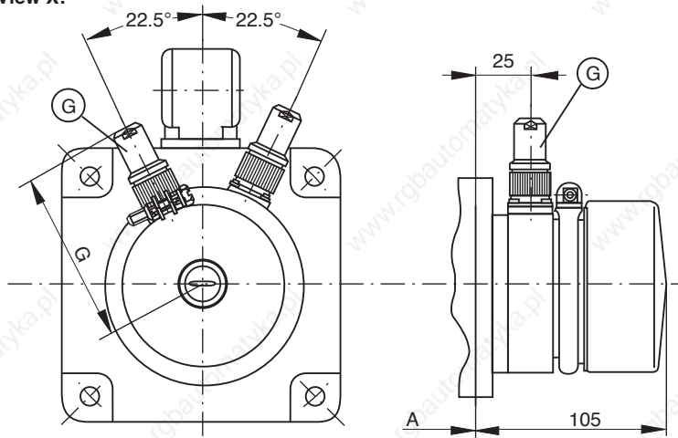
View X:
