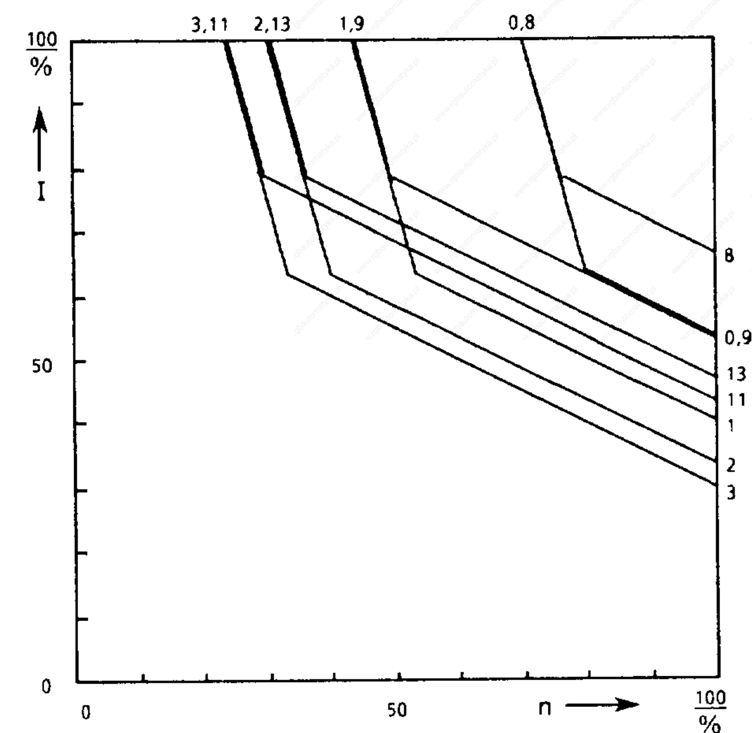
Fig. 3.2 Adjustable characteristics of speed-dependent current limitation
