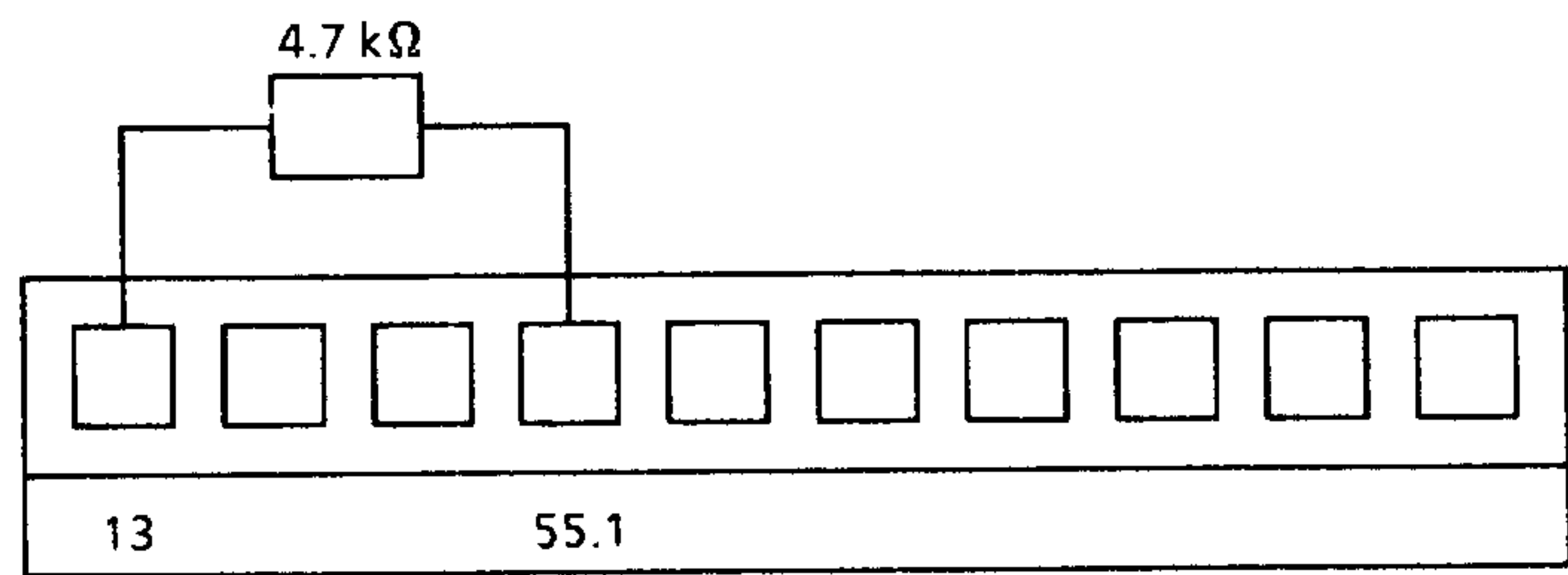
Fig. 3.10 Connector X1.1
