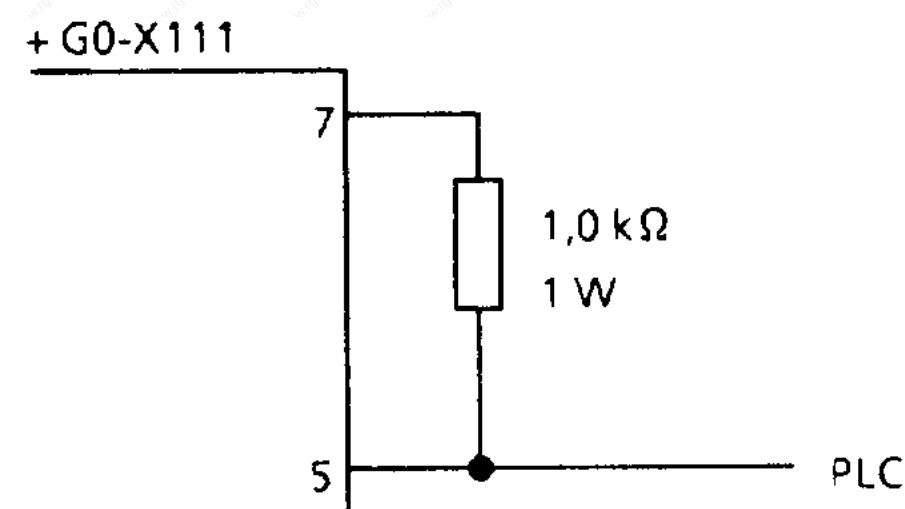
Fig. 3.13 Connection to the PLC resistor only necessary with power supplies 6SC6100-0GA00 and -0GB00
