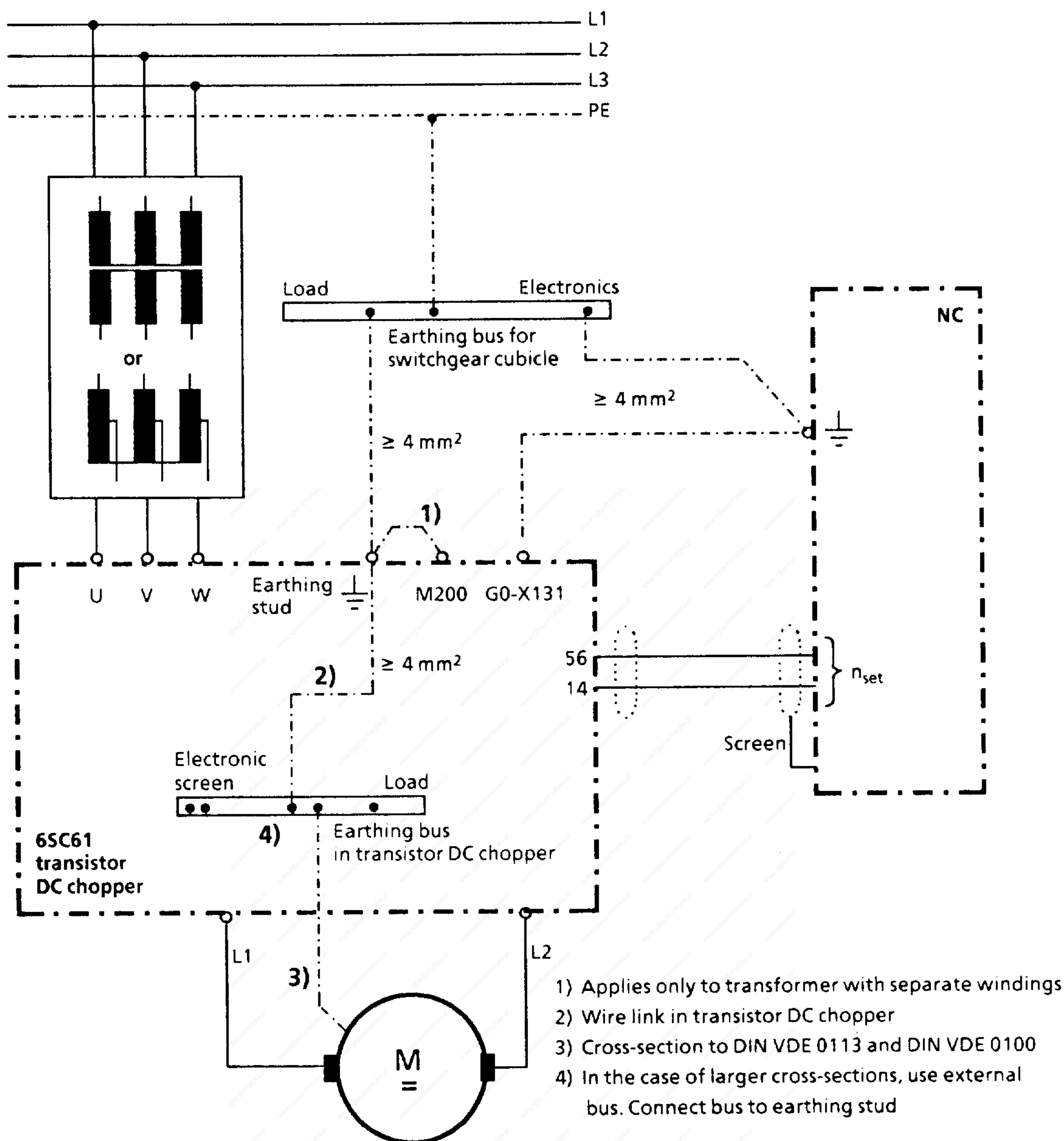
Fig. 2.1 Earthing concept
