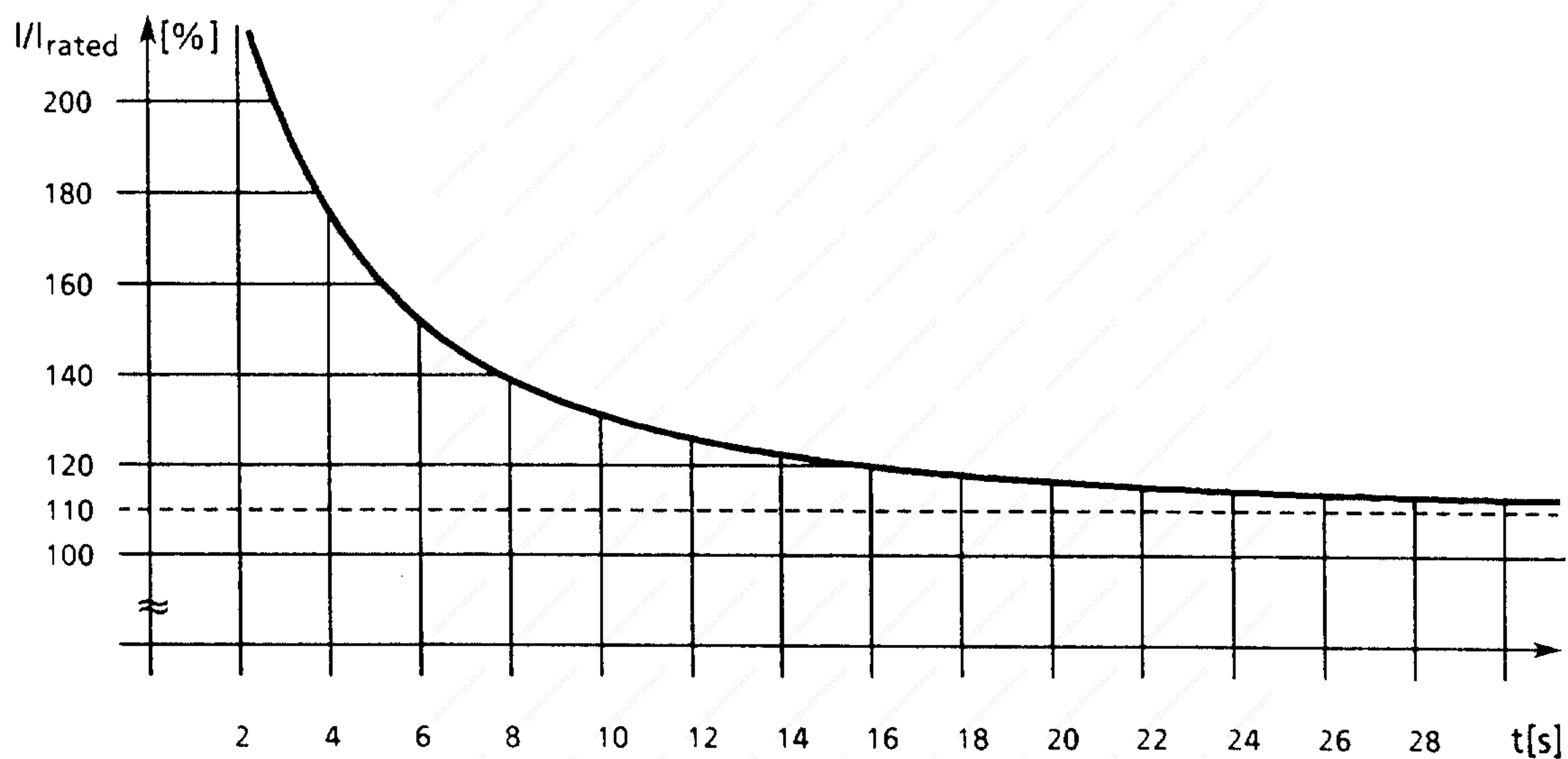
Fig. 3.11 I^2t curve \hat{=} thermally permissible time duration of overcurrent
