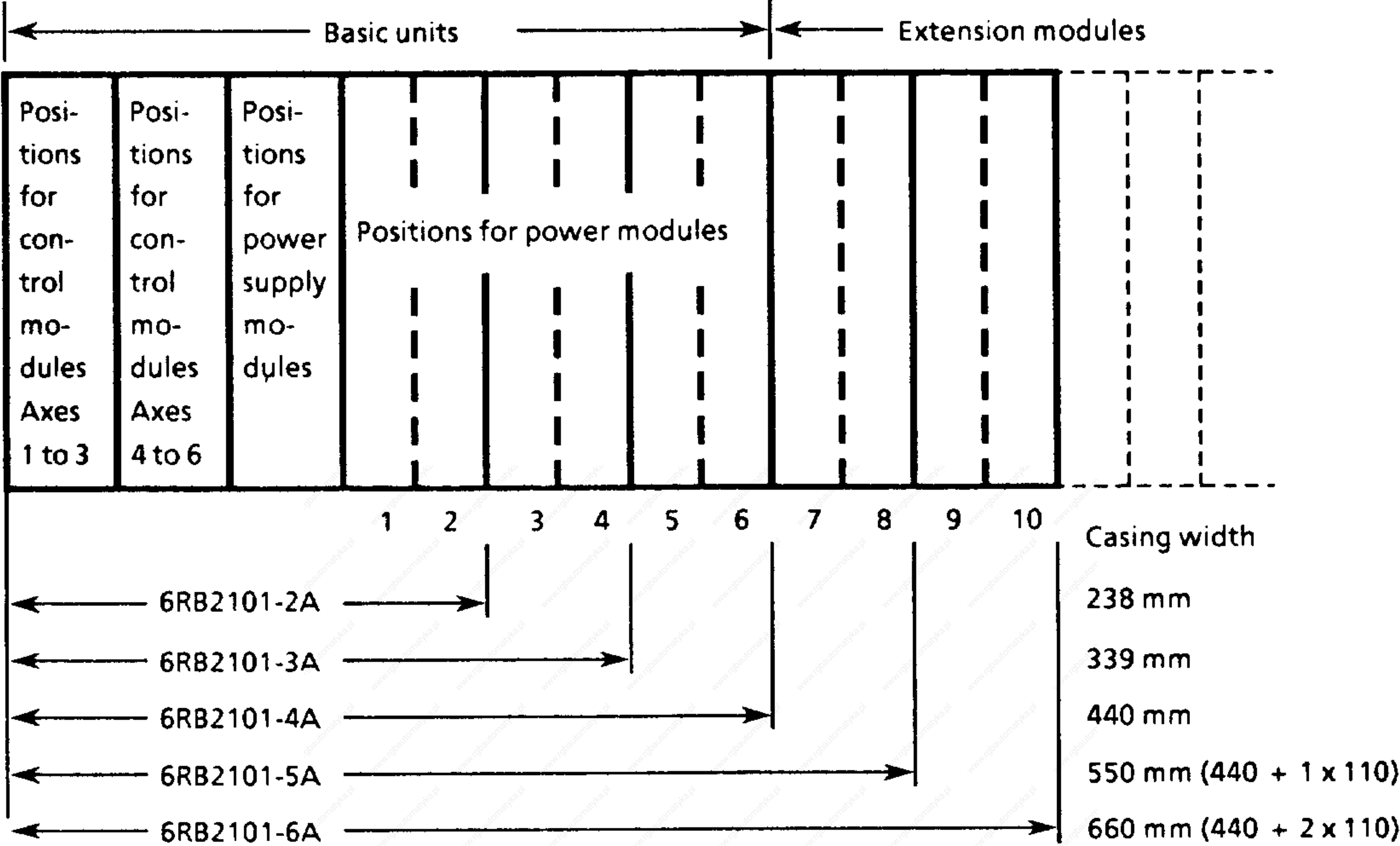
Fig. 1.2 Casing
