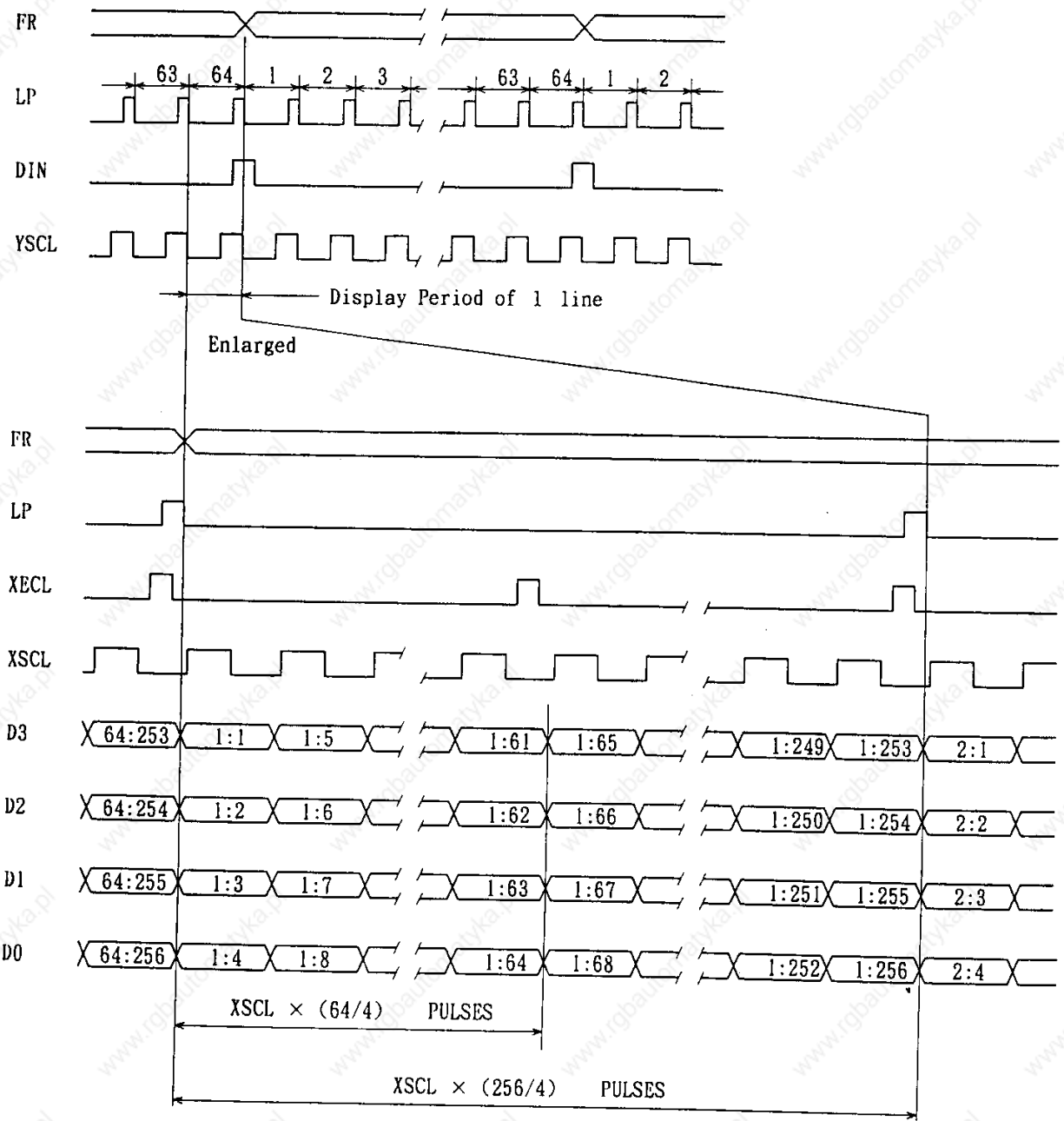
3-4 Timing Chart 2
