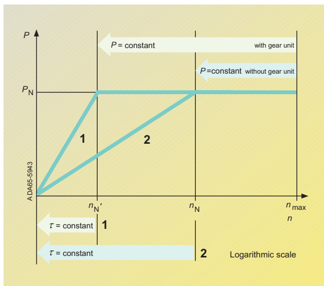
Fig. 4/9 Speed/power graph
