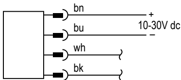
Emitters with Quick Disconnect (4-pin Euro-Style)
