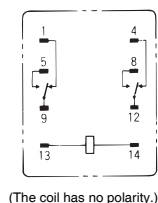
Terminal Arrangement/Internal Connections (Bottom View) Standard Models
