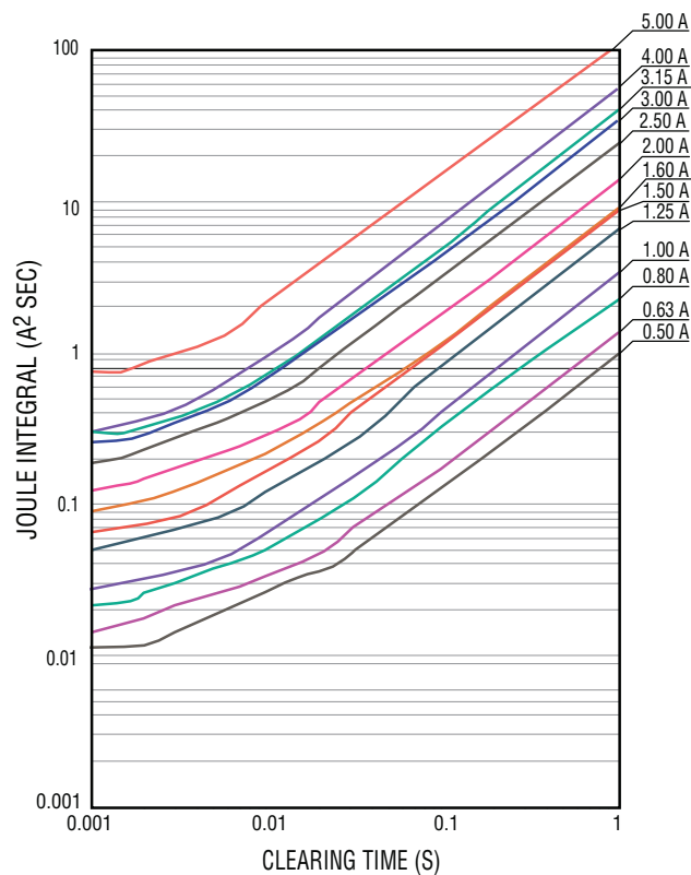
Minimum I²T V Clear Time Curves
