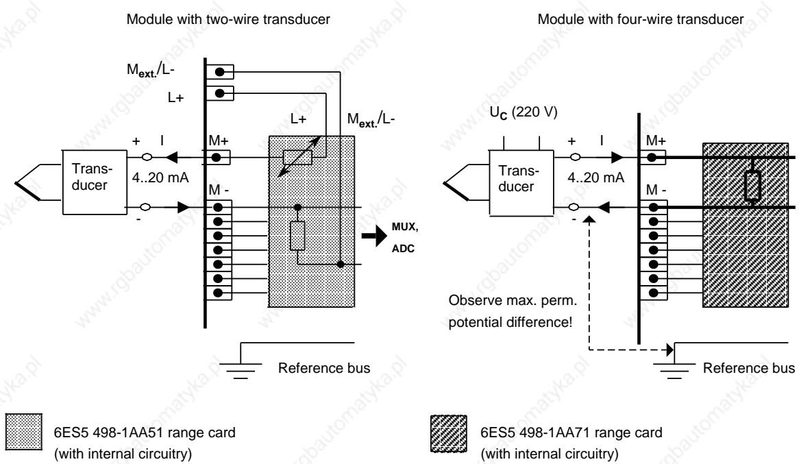
Figure 10-8. Connecting Transducers
