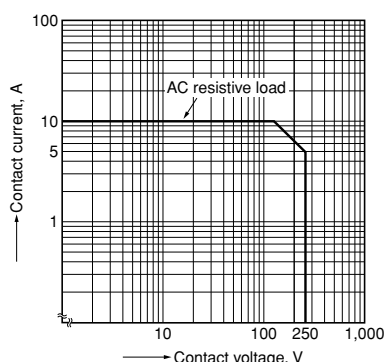
1.-(1) Max. switching capacity (1 Form A type)
