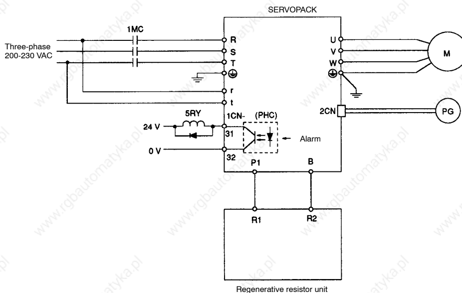
Connecting a Regenerative Resistor Unit
