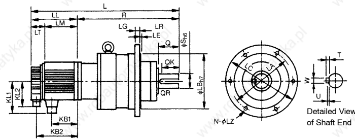
Grease-lubrication type large size servomotors
