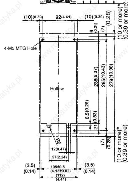
Mounting Surface Diagram
