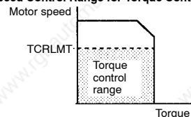
Speed Control Range for Torque Control
