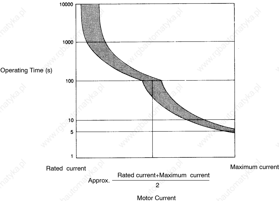
Overload Characteristics
