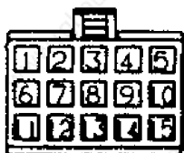
Encoder plug
