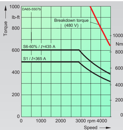
1PL6224-4.L. max. breakdown torque: 1490 lb-ft/2021 Nm
