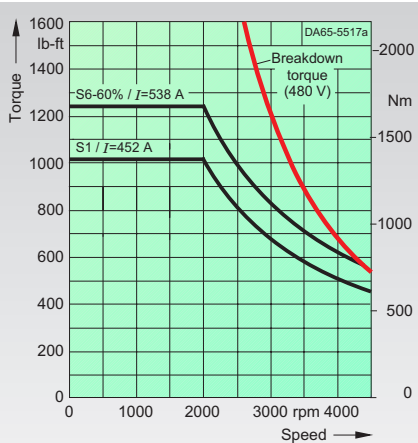
1PL6228-4.F. max. breakdown torque: 2646 lb-ft/3687 Nm
