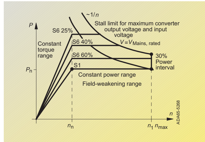
Fig. 3/4 Power-speed characteristic
