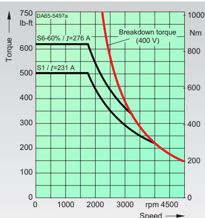
1PL6186-4.F. max. breakdown torque: 1210 lb-ft/1640 Nm
