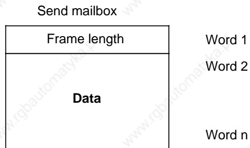
Figure 12-19. Structure of the Send Mailbox
