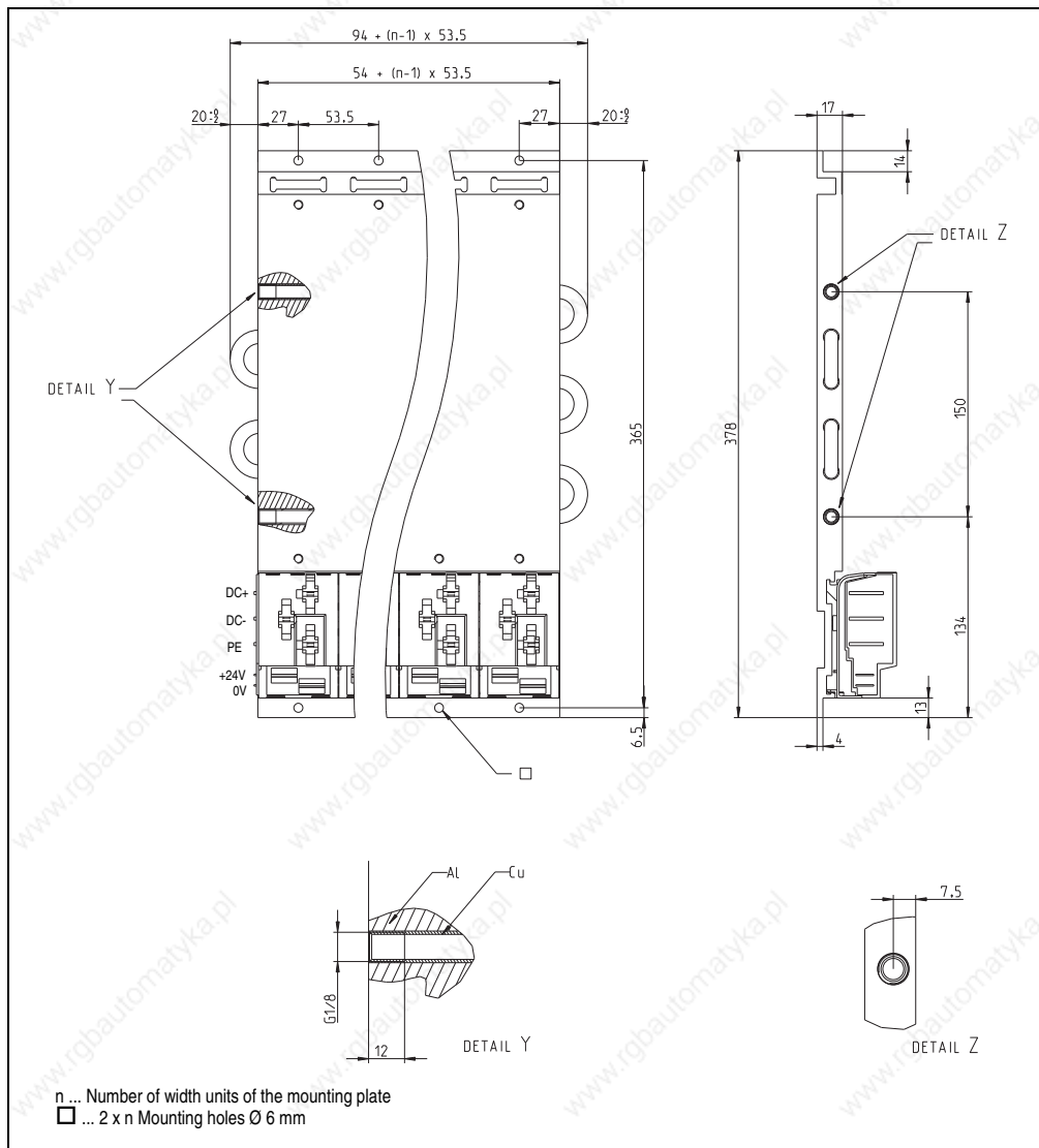
Figure 50: Dimension diagram and installation dimensions - 8B0MnnnnHC00.000-1
