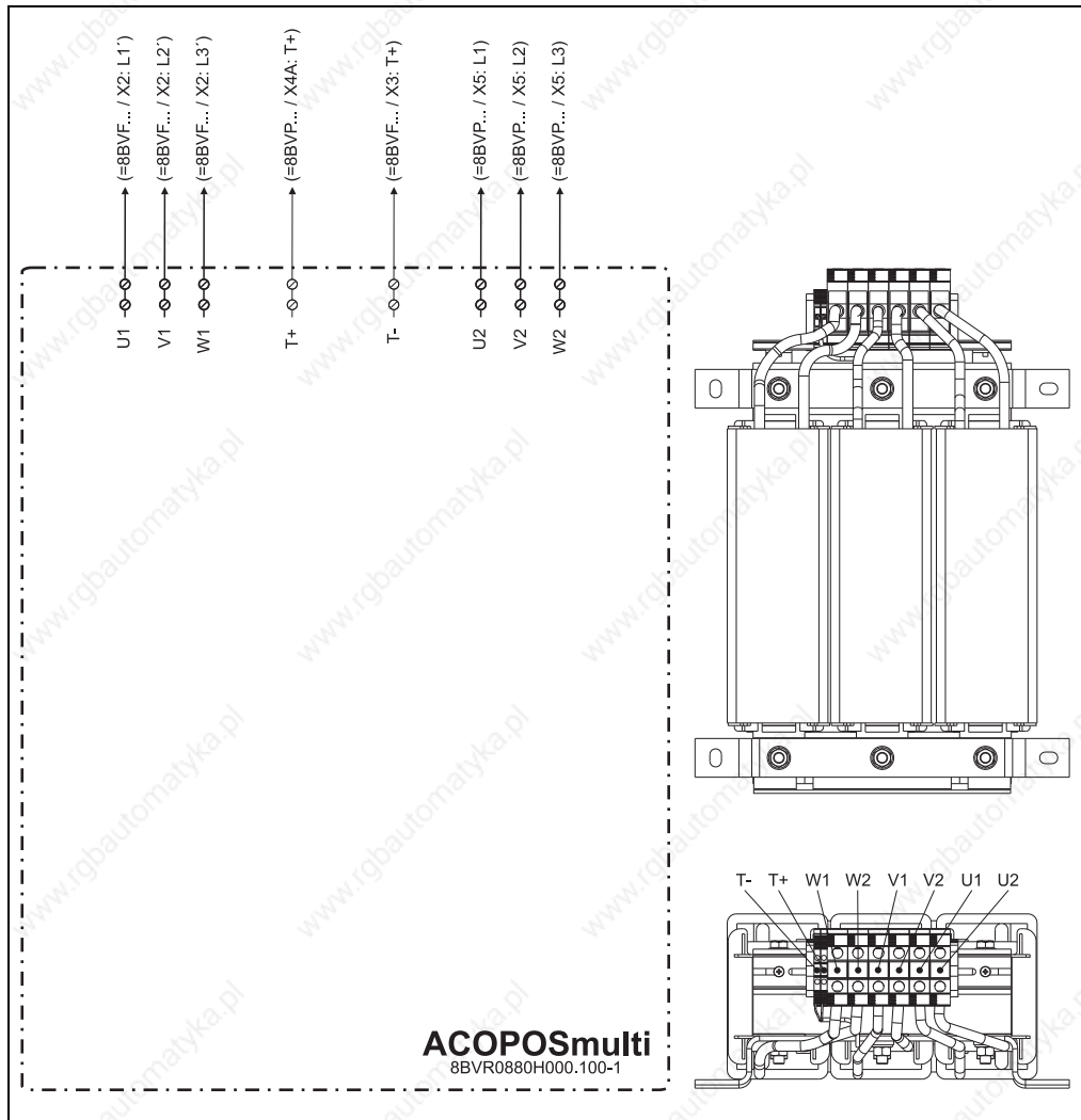
Figure 123: Overview of pin assignments - 8BVR0880H000.100-1
