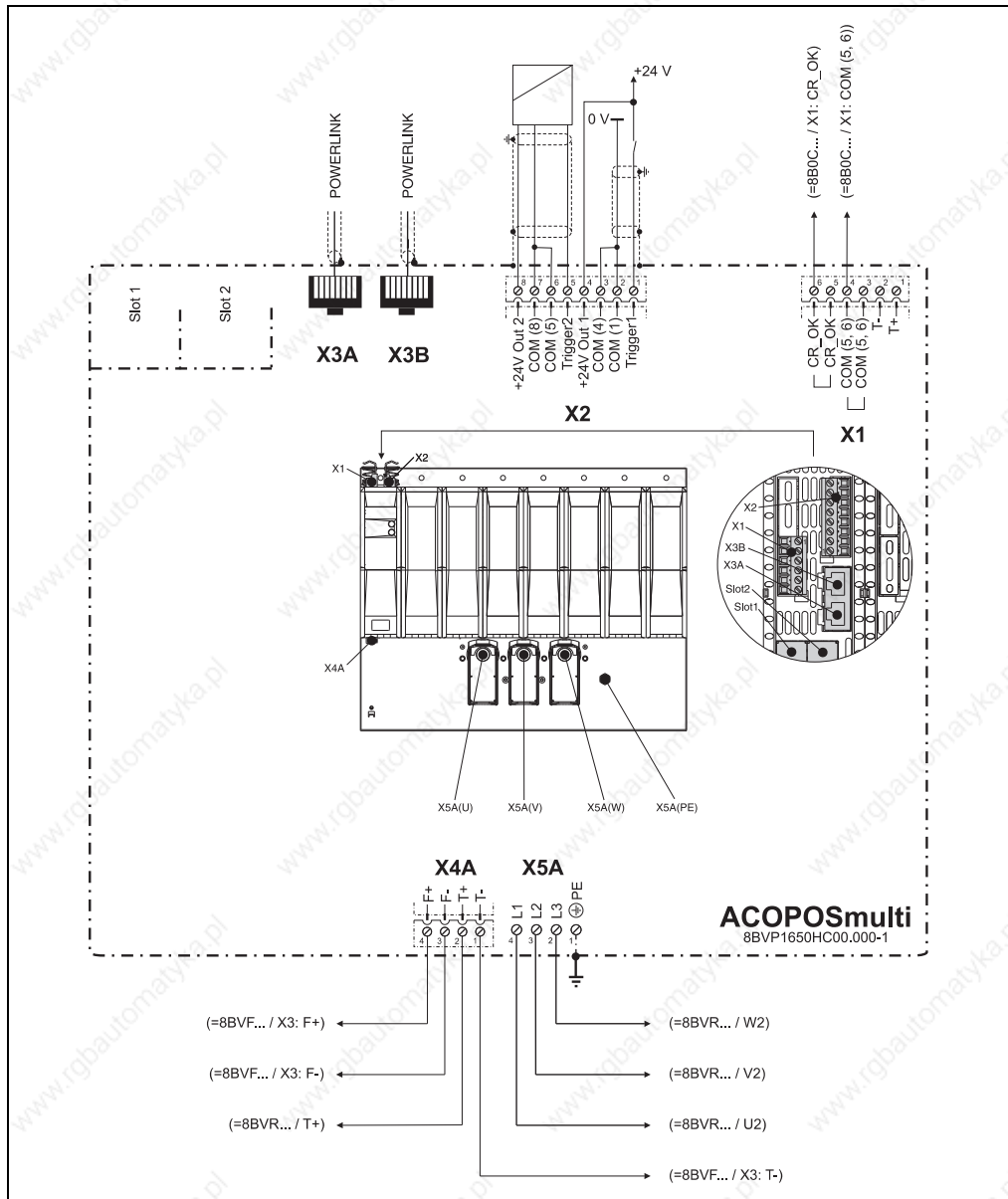
Figure 134: Overview of pin assignments - 8BVP1650HC00.000-1
