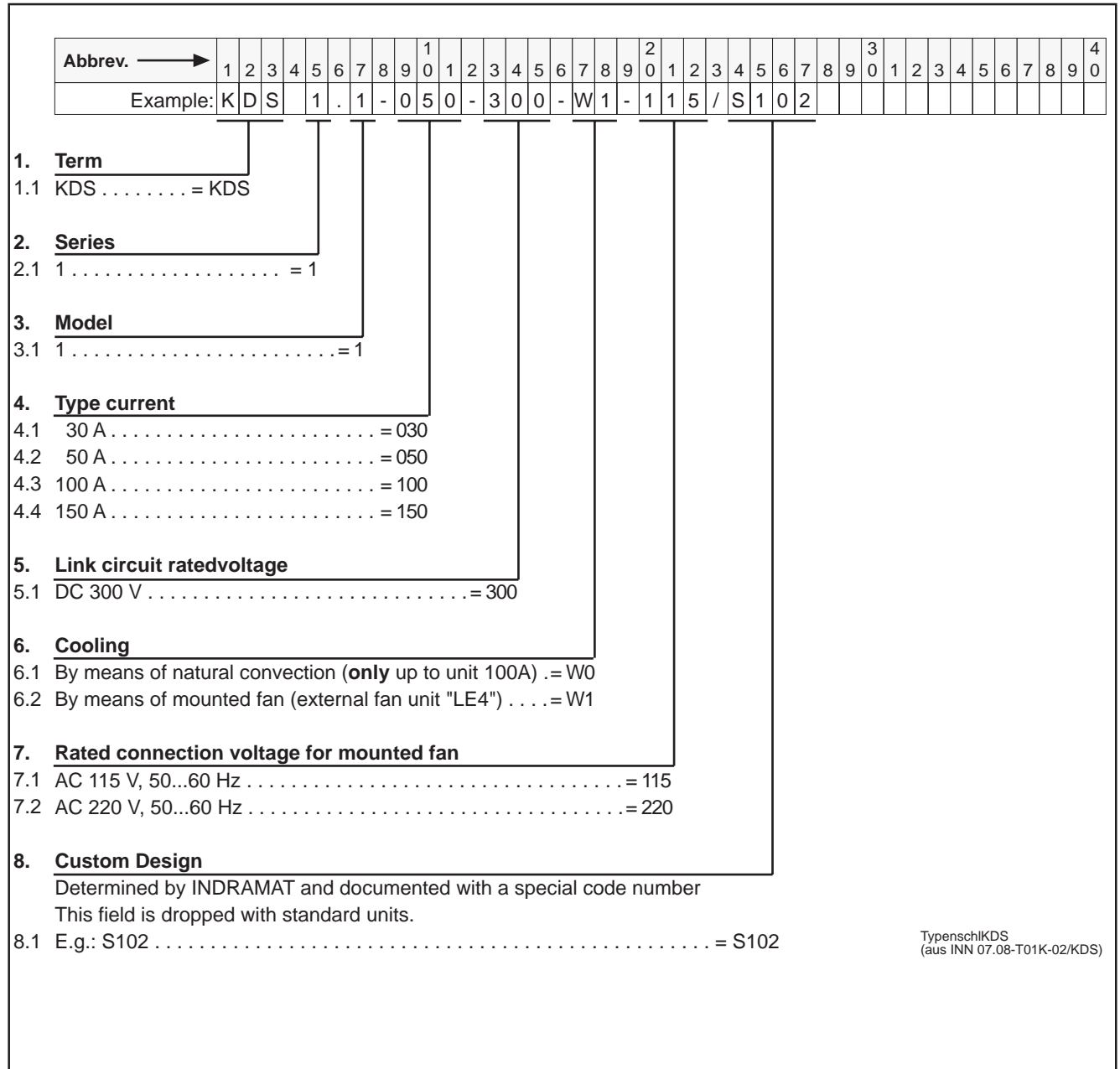
Figure 114: Type codes for KDS servo-drive module
