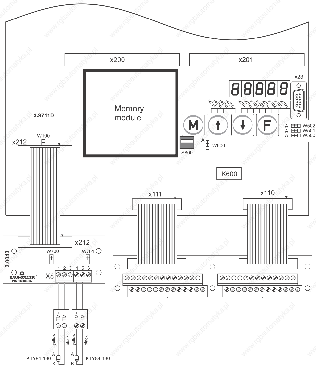
Illustration 87: Connection option board 3.0043
