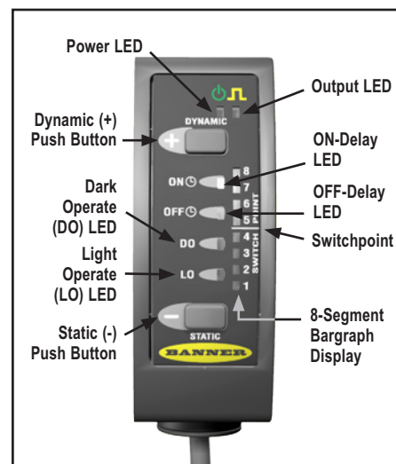
Figure 1. Sensor features
