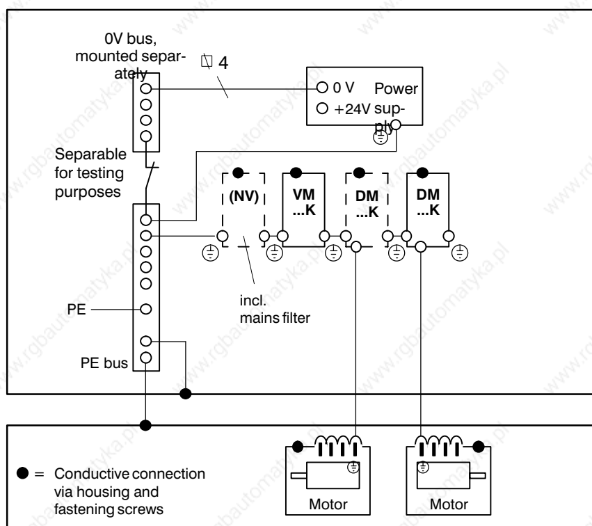
Fig. 2.7: Earthing plan Servodyn-D with VM...K
