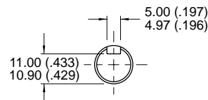
KEYWAY DETAIL
