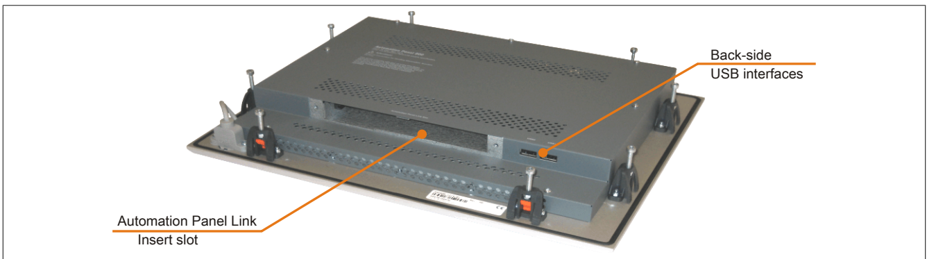
Figure 41: 5AP920.1214-01 - Rear view
