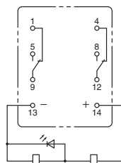
MY2IN(S) (DC Models)
