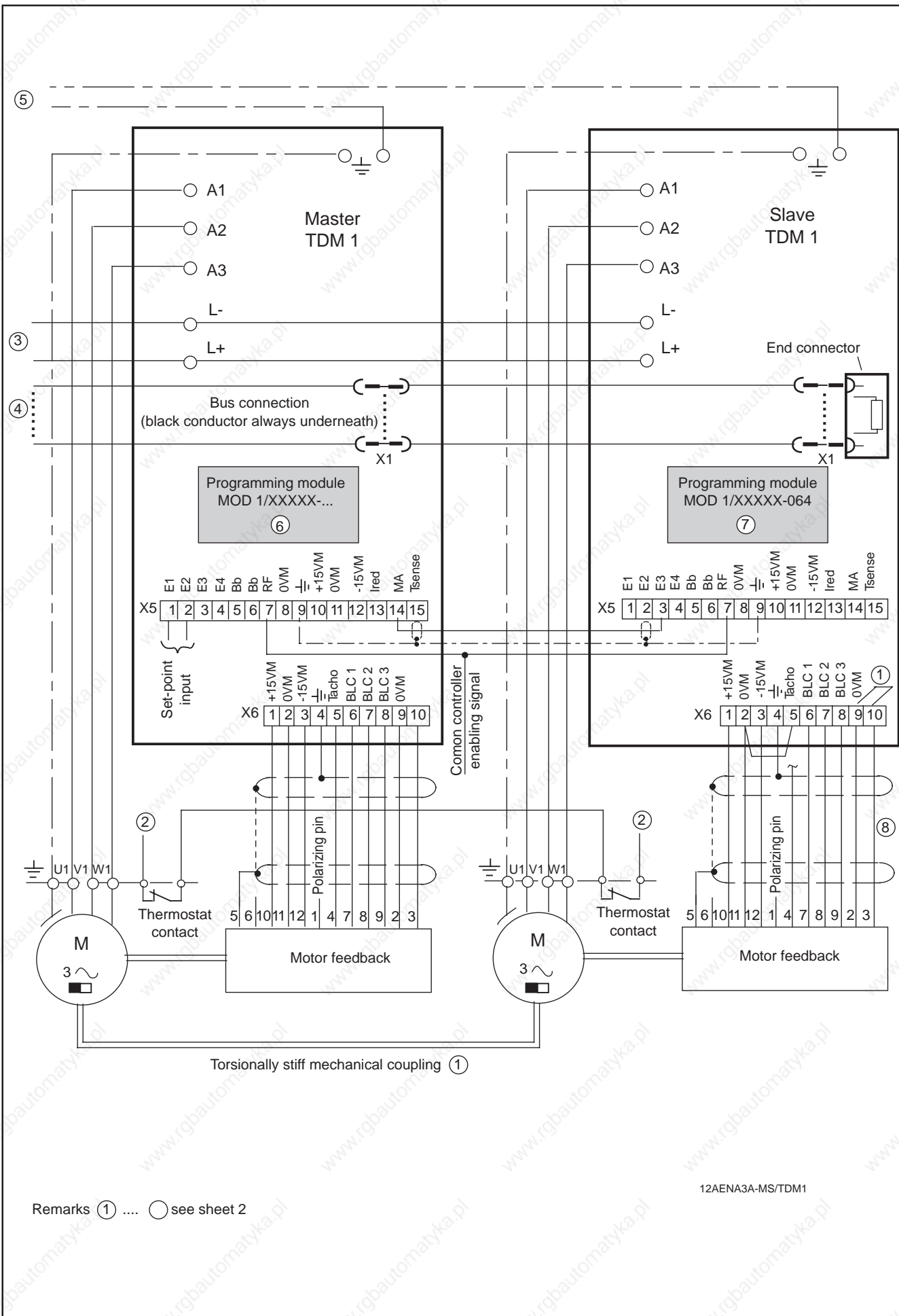
Fig. 12: Connection diagram for master-slave drive with TDM 1
