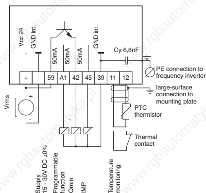
Connection with internal power supply
