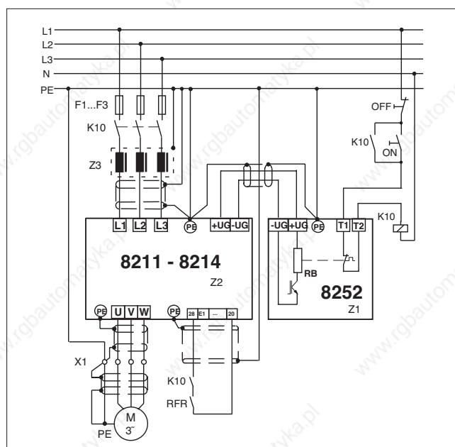
Connection example with brake module
