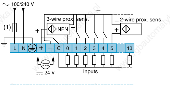
Negative logic
