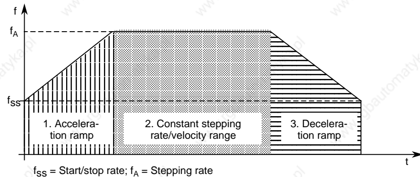
Figure 15-29. Velocity Profile of the IP 267
