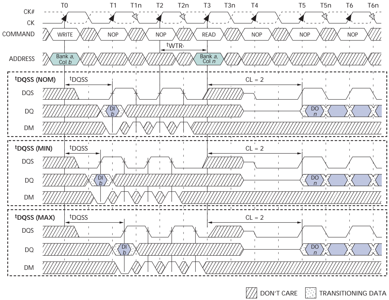
Figure 44: WRITE-to-READ – Odd Number of Data, Interrupting
