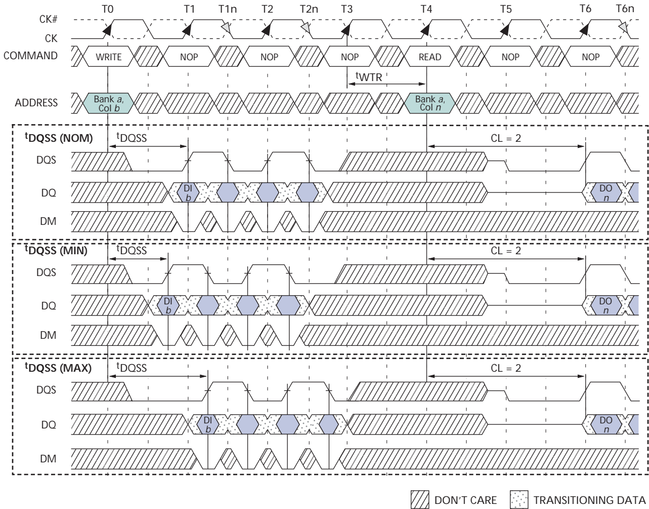
Figure 42: WRITE-to-READ – Uninterrupting
