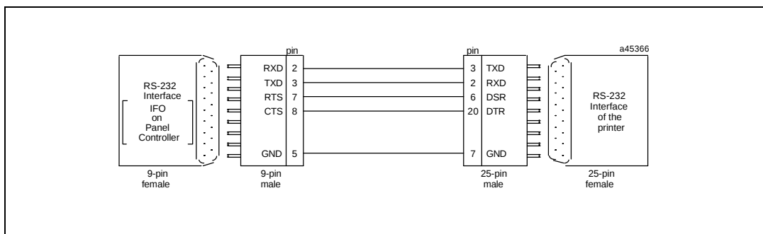
Figure 7 - 3. Serial Printer Cable Connections
