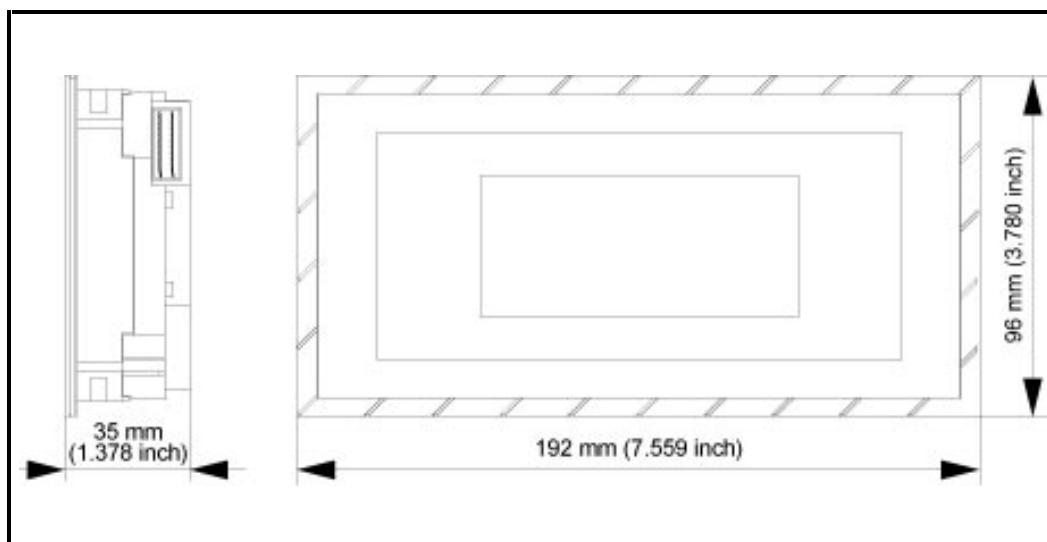
Figure 3 - 4. Display Module with 4 X 20 LCD
