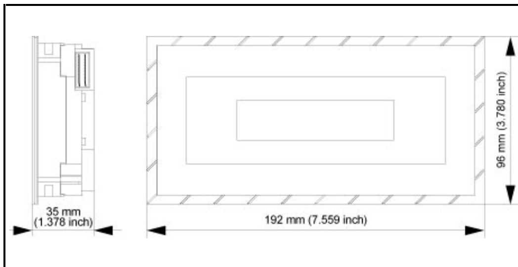
Figure 3 - 3. Display Module with 2 X 20 LCD
