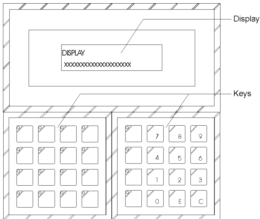
Figure 1 - 1. Interface Panel Components
