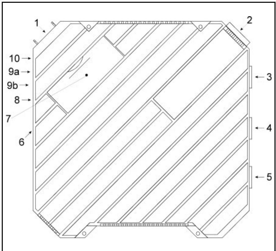
Figure 5 - 2. Basic Panel Controller (C200) Elements/Connections
