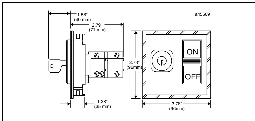
Figure 4 - 10. Key Switch Module
