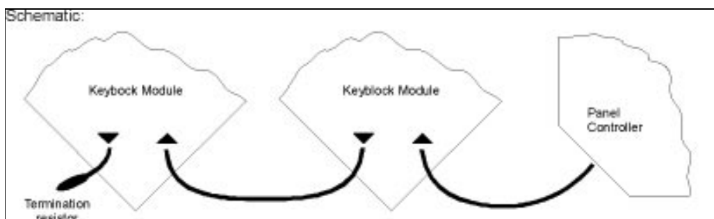
Figure 4 - 2. Keyblock Module Connection Schematic
