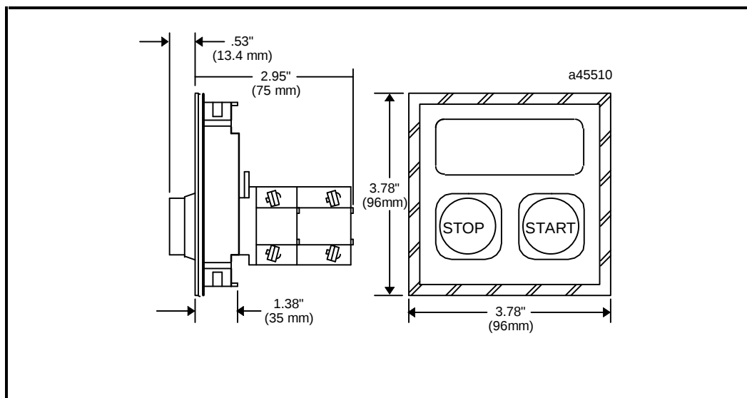
Figure 4 - 11. Start/Stop Module
