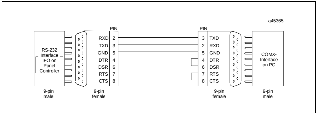
Figure A - 3. Serial Connection Between Controller and PC
