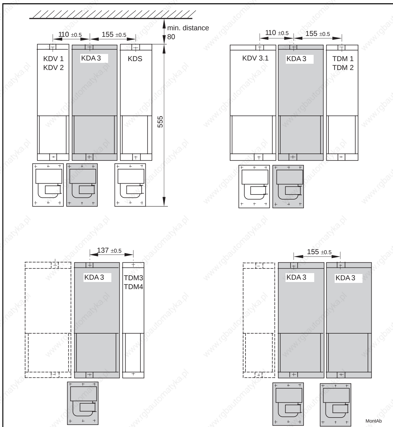
Fig 2.6 Installation distances upwards and to adjacent units of the drive
