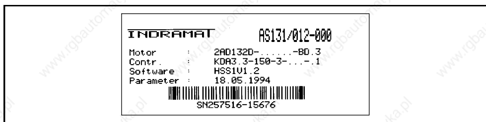
Fig 3.1 Programming module AS with rating plate
