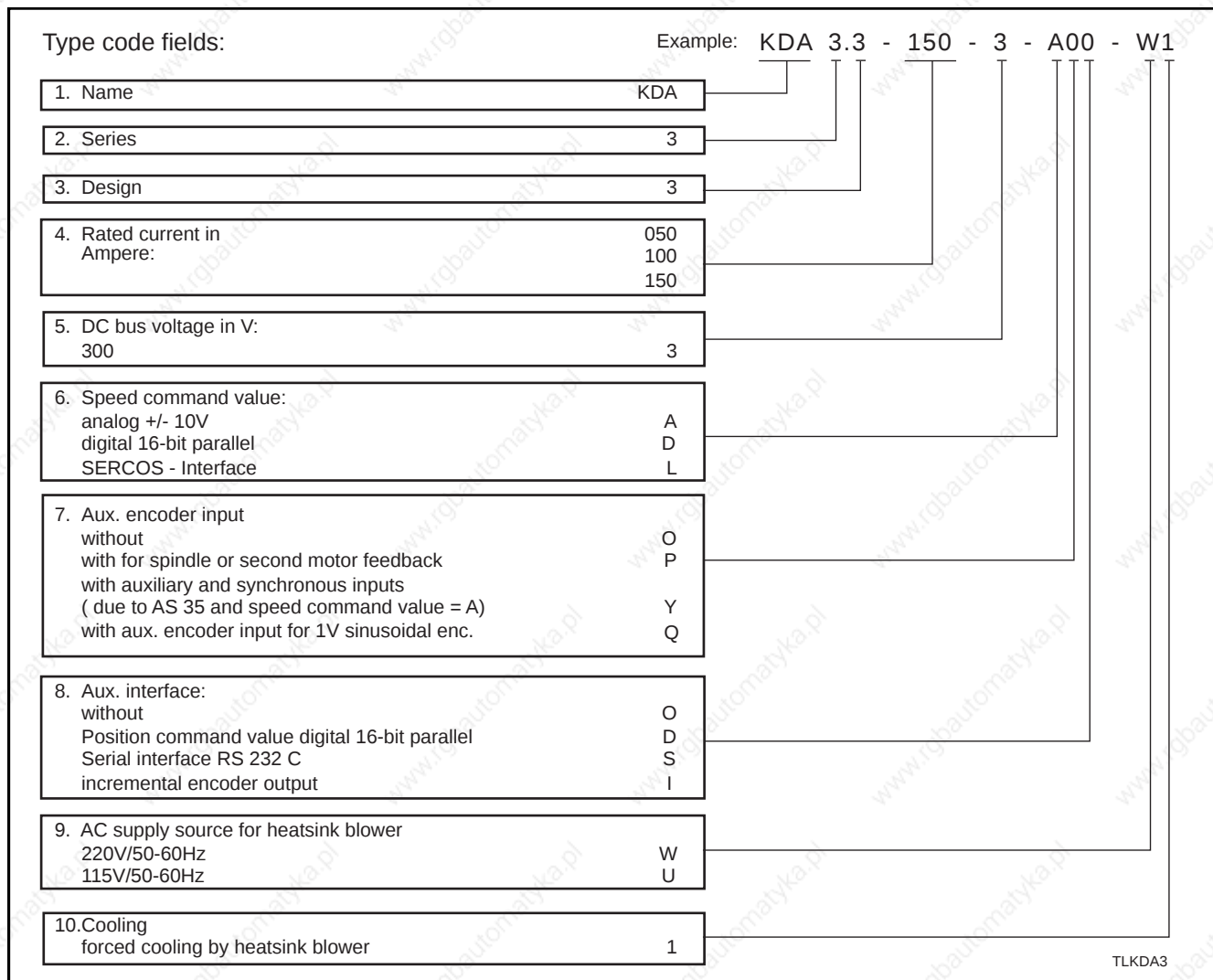
Fig 2.16 KDA - type codes
