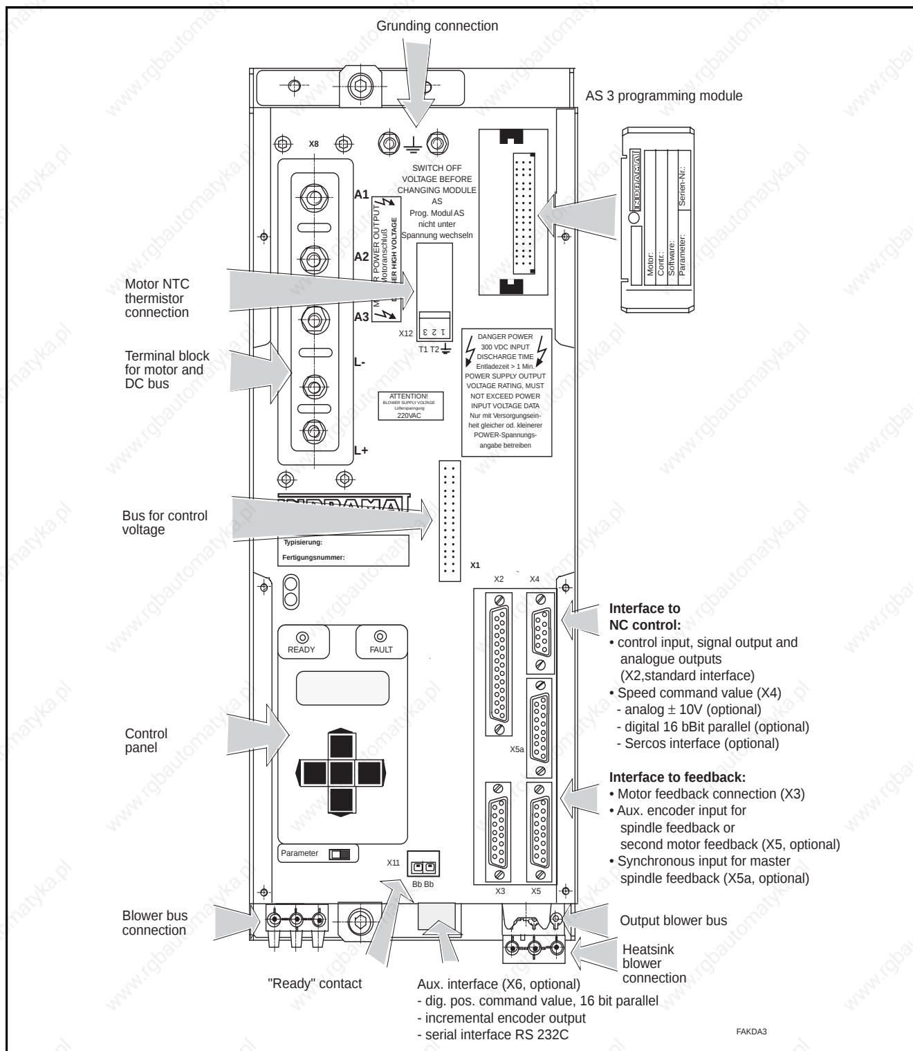
Fig 1.4 Definition allocation on KDA 3
