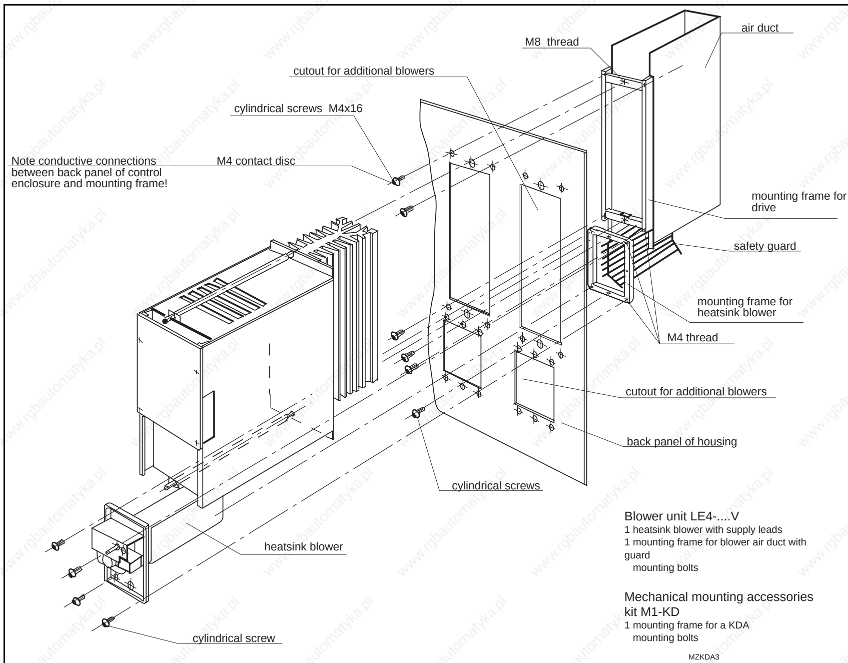
Fig 7.1 Installation of unit
