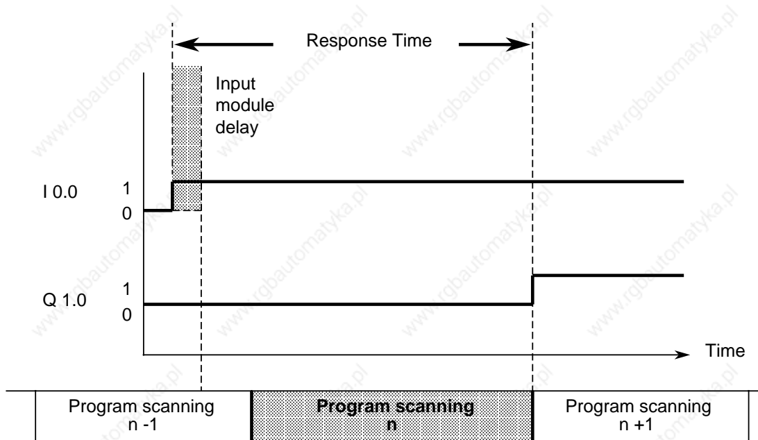
Figure 2-15. Response Time
