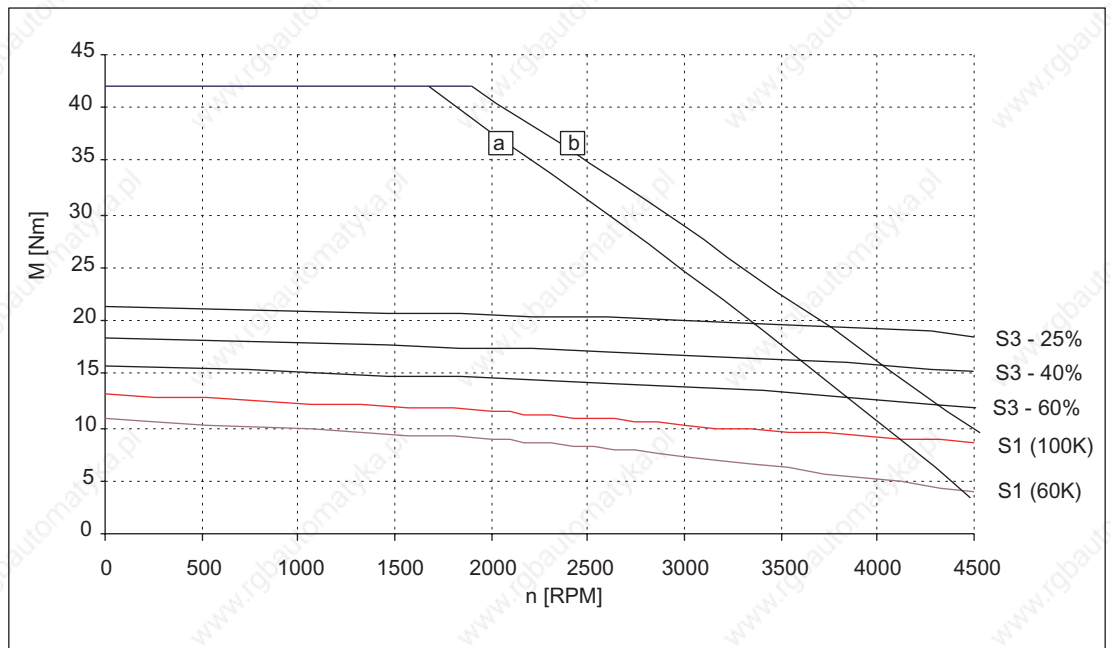
Figure 3-26 Speed-torque diagram 1FT6082-8AF7□
