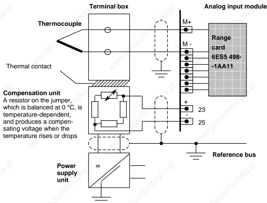
Figure 10-4. Connecting Thermocouples
