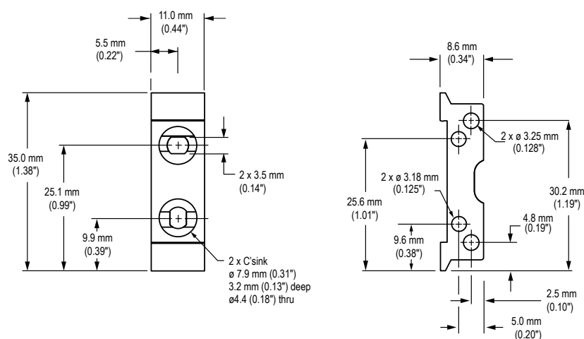
Figure 3. Mounting Bracket
