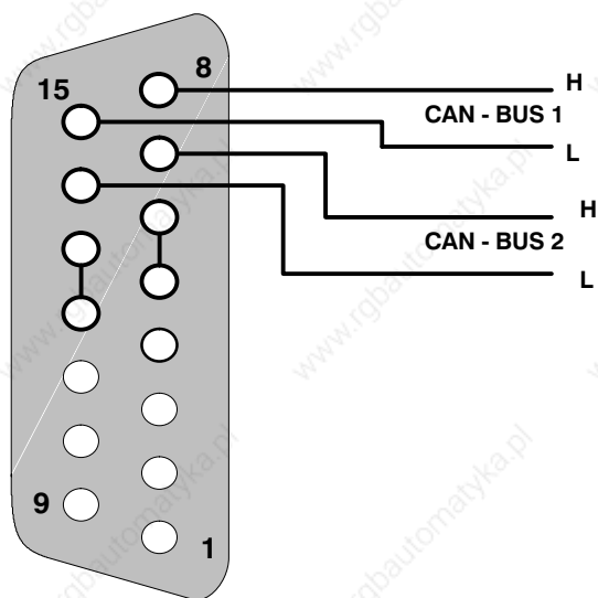
2 CAN - bus systems with bus termination on the rho 3 - CAN - connector
