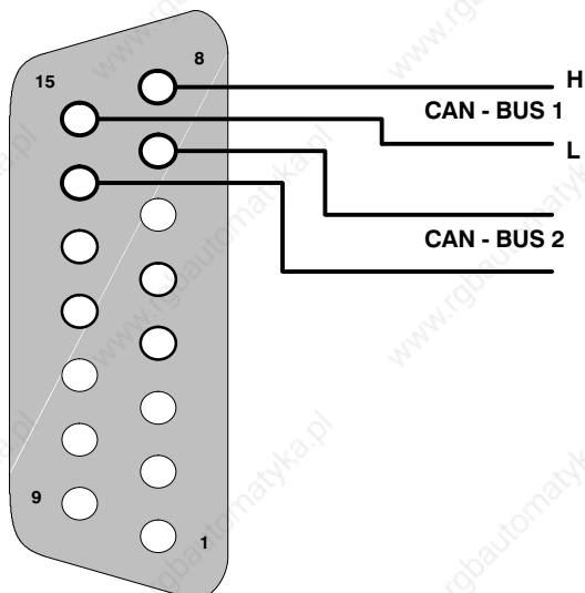
2 CAN - bus systems without bus termination
