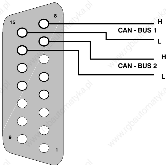
2 CAN - bus systems without bus termination the bus termination is implemented on the other bus station
