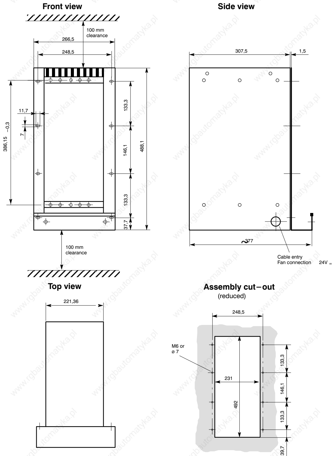
RC-Card-Rack 2.5 - 6
