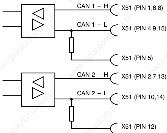
Pin assignment (CAN bus interface)
