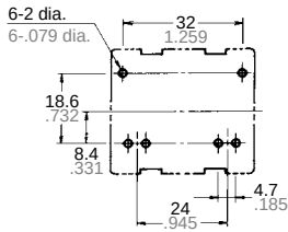
PC board pattern (Copper-side view)
