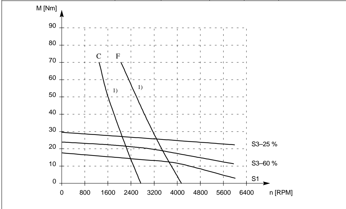
Fig. 2-33 Speed–torque diagram, 1FT5101
