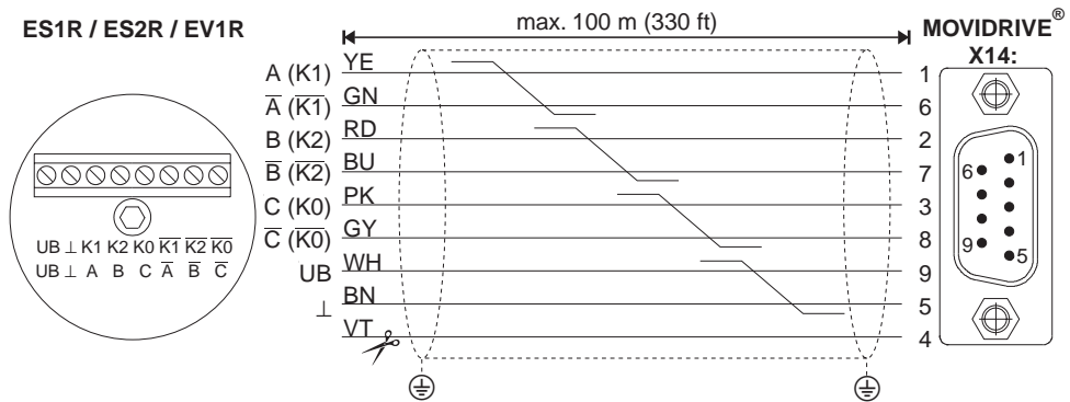
Fig. 40: External encoder direct to X14:
