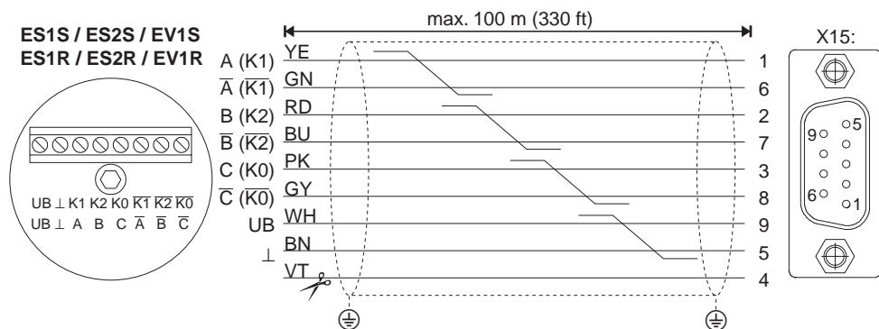
Fig. 33: Connecting the sin/cos encoder
