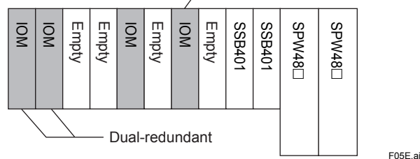
Figure Example Mounting of I/O Module on Safety Node Unit
