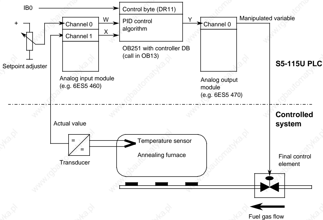
Figure 11-5. Process Schematic
