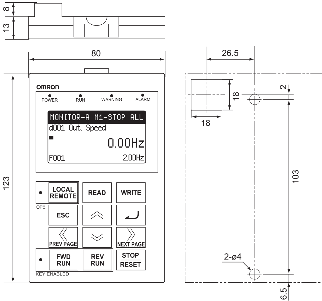
External Appearance of the LCD Digital Operator
