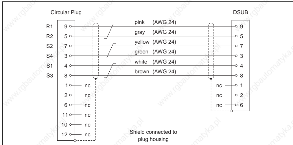
Figure 70: Cable schematic for resolver cables
