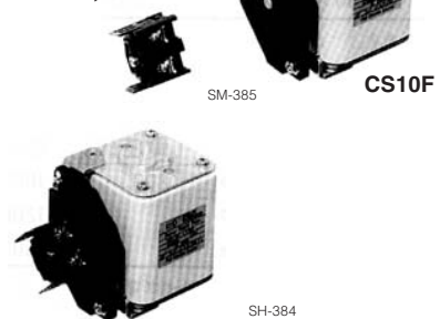
CS 10F with alarm contact block
