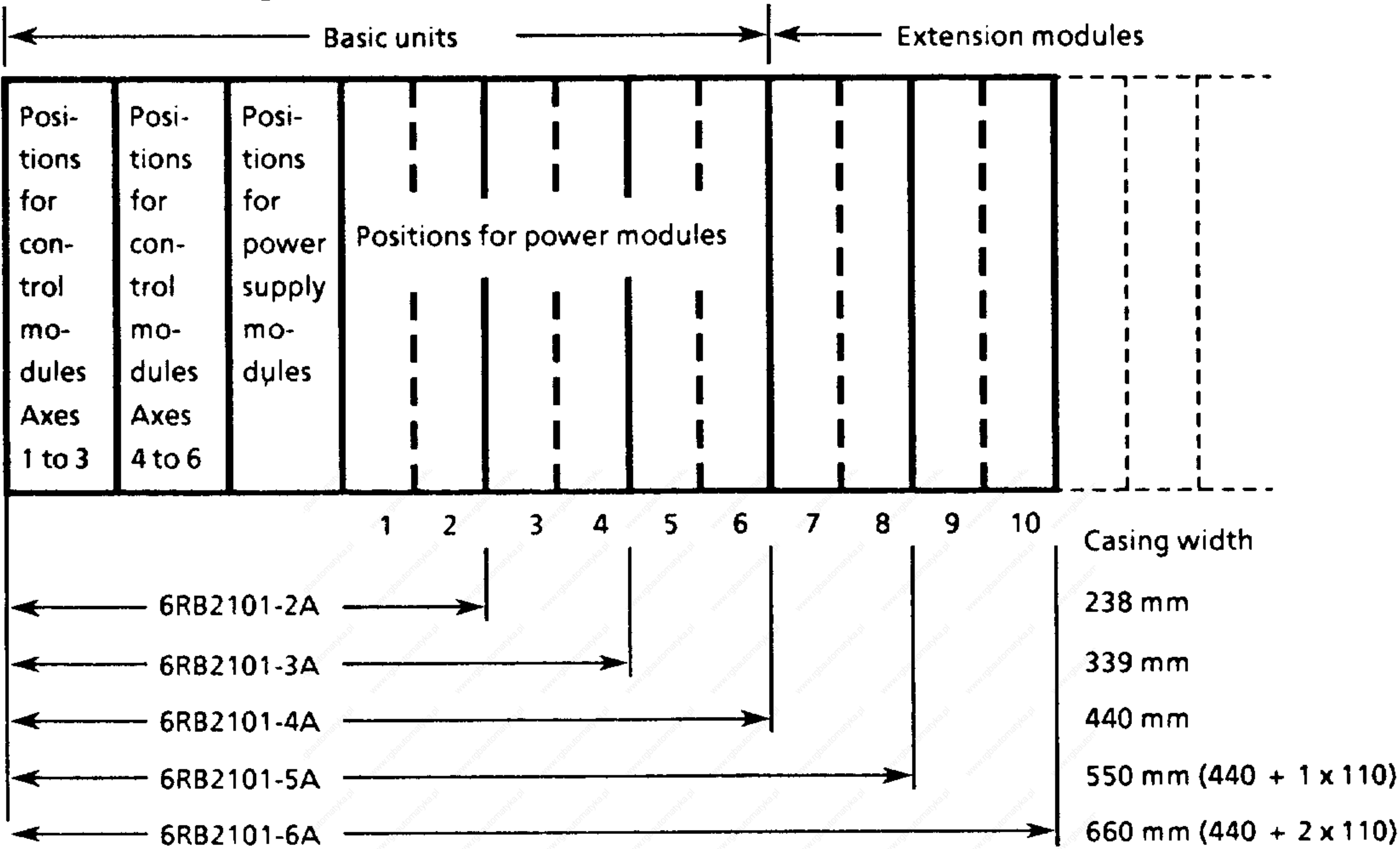
Fig. 1.2 Casing
