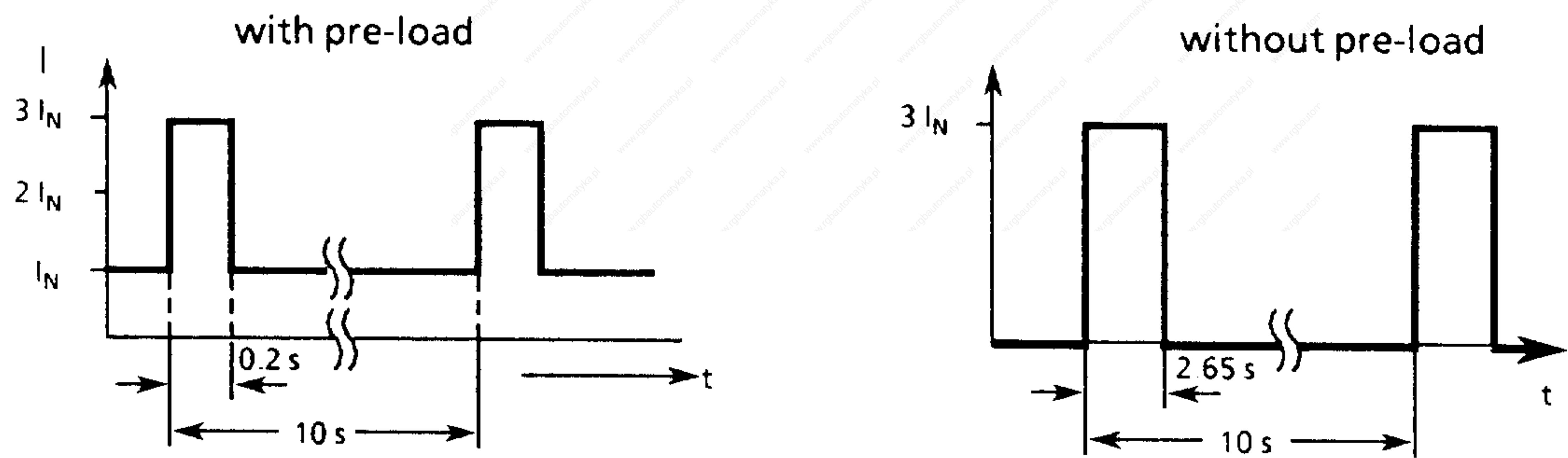
Fig 1.3 Rated load cycles for power modules in operation with short-time limit current
