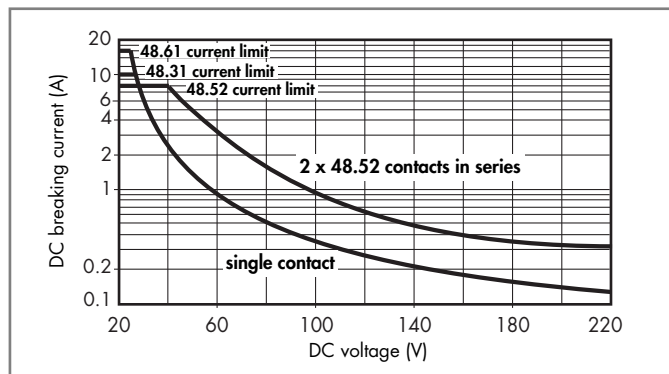
H 48 - Maximum DC1 breaking capacity Types 48.31/52/61
