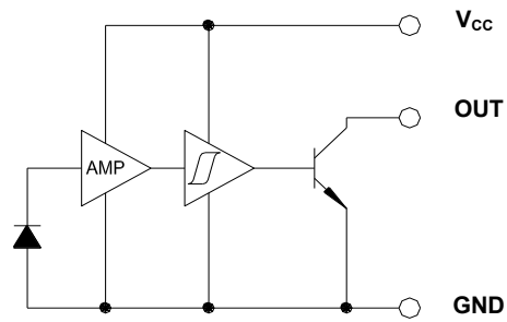
OPL531A, OPL536/536A Inverted 10K Pull-Up
