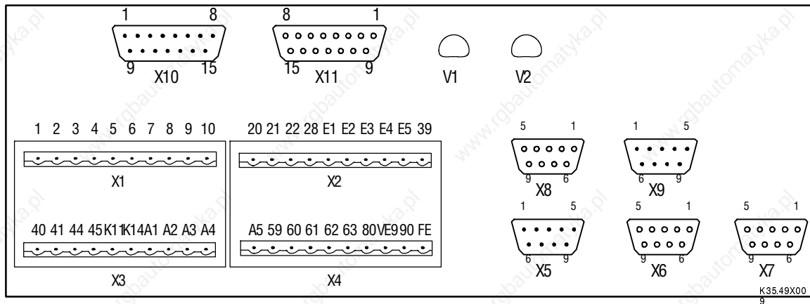
FIG 4-8 Control connections for the controller
