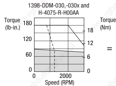
1398-DDM-030 1398-DDM-030x
