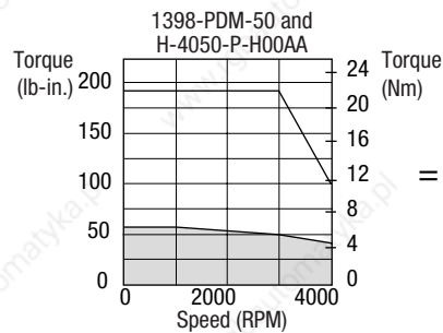
1398-PDM-50
