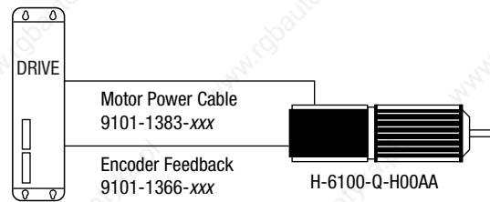
1398-DDM-075 1398-DDM-075x
