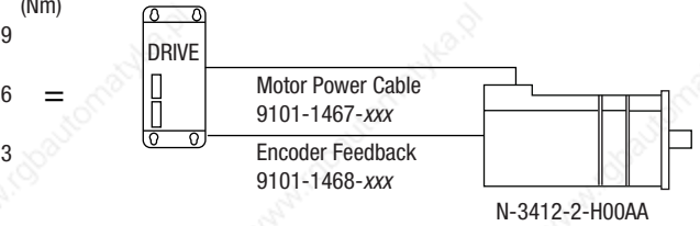
1398-DDM-009 1398-DDM-009x
