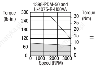
1398-PDM-50
