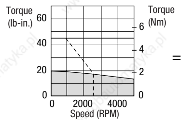
1398-DDM-020,-020x and H-3016-N-H00AA
