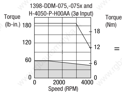
1398-DDM-075 1398-DDM-075x
