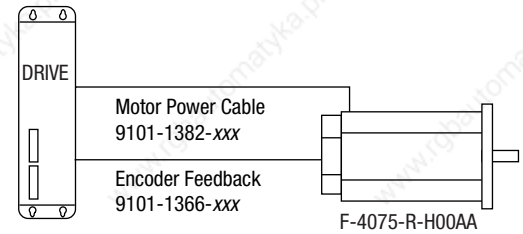
1398-DDM-030 1398-DDM-030x
