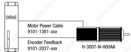
1398-PDM-10
