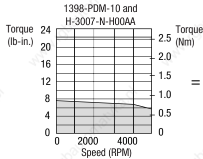
1398-PDM-10
