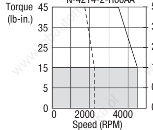
1398-DDM-009,-009x and N-4214-2-H00AA
