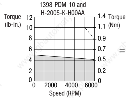
1398-PDM-10
