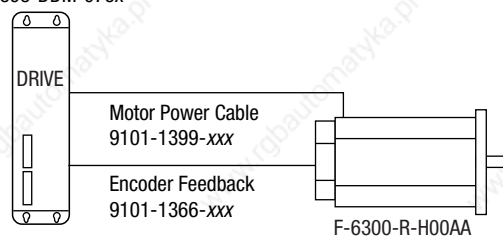
1398-DDM-075 1398-DDM-075x
