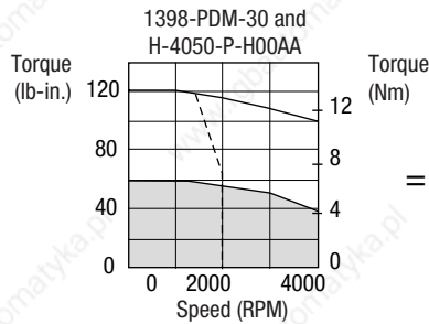
1398-PDM-30
