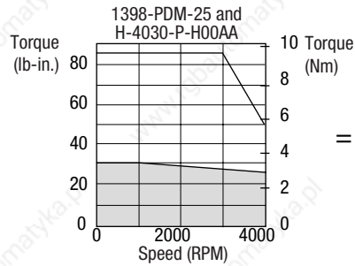
1398-PDM-25
