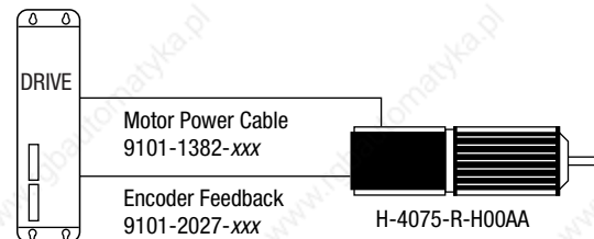
1398-PDM-30
