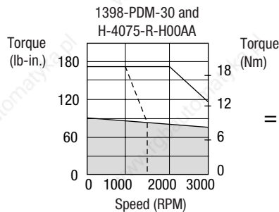
1398-PDM-30
