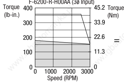
1398-DDM-075,-075x and F-6200-R-H00AA (3Ø Input)
