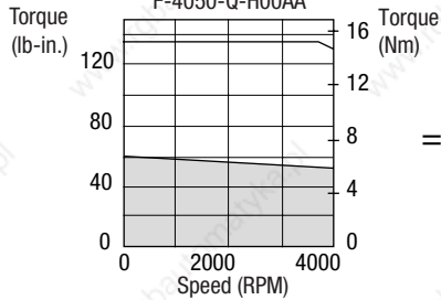
1398-PDM-50 and F-4050-Q-H00AA
