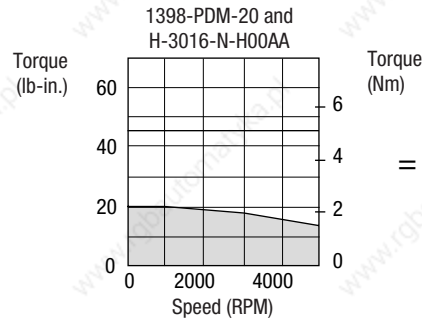
1398-PDM-20
