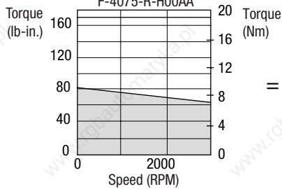
1398-PDM-50 and F-4075-R-H00AA
