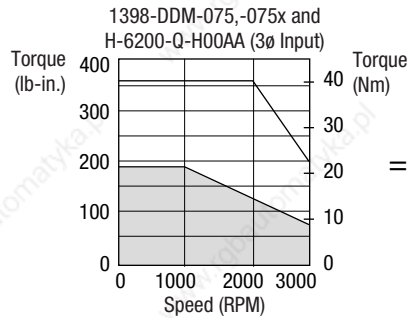
1398-DDM-075 1398-DDM-075x
