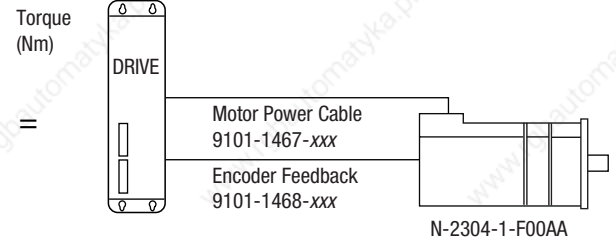
1398-DDM-009 1398-DDM-009x
