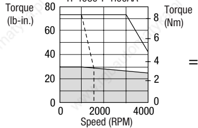
1398-DDM-020,-020x and H-4030-P-H00AA
