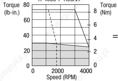
1398-DDM-019,-019x and H-4030-P-H00AA
