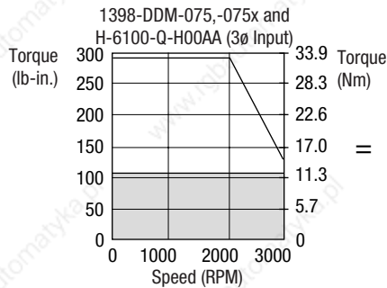
1398-DDM-075 1398-DDM-075x
