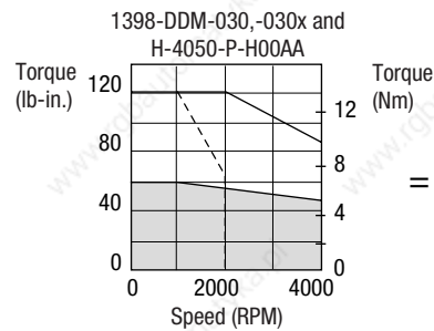
1398-DDM-030 1398-DDM-030x
