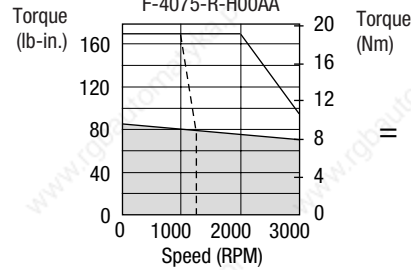
1398-DDM-075,-075x and F-4075-R-H00AA (3Ø Input)
