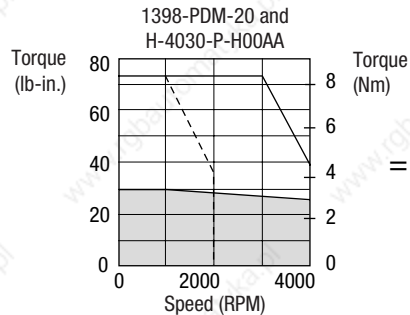
1398-PDM-20
