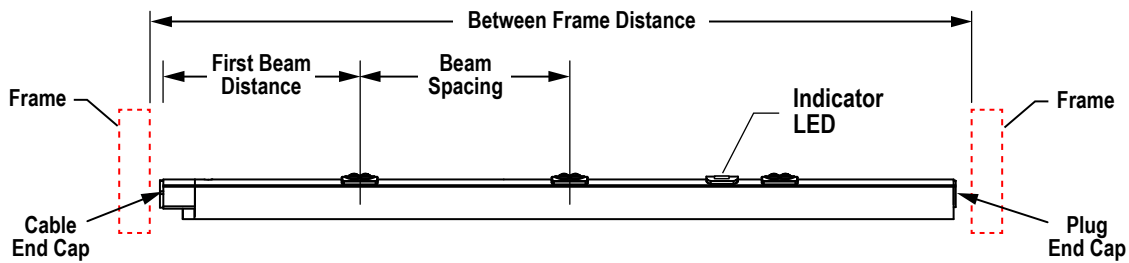
Figure 2. T-Slot Configuration
