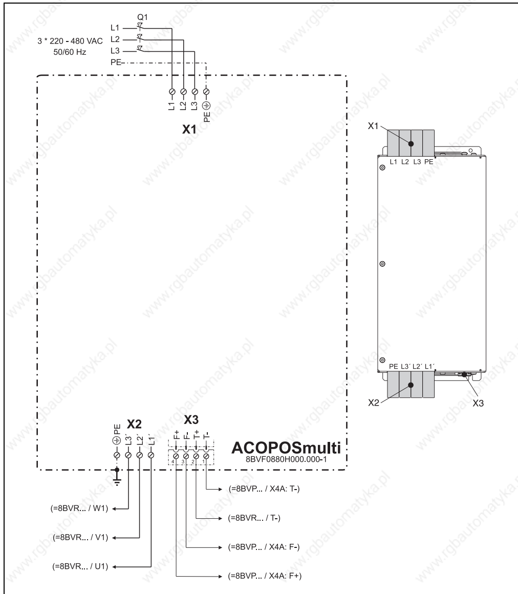
Figure 117: Overview of pin assignments - 8BVF0880H000.000-1
