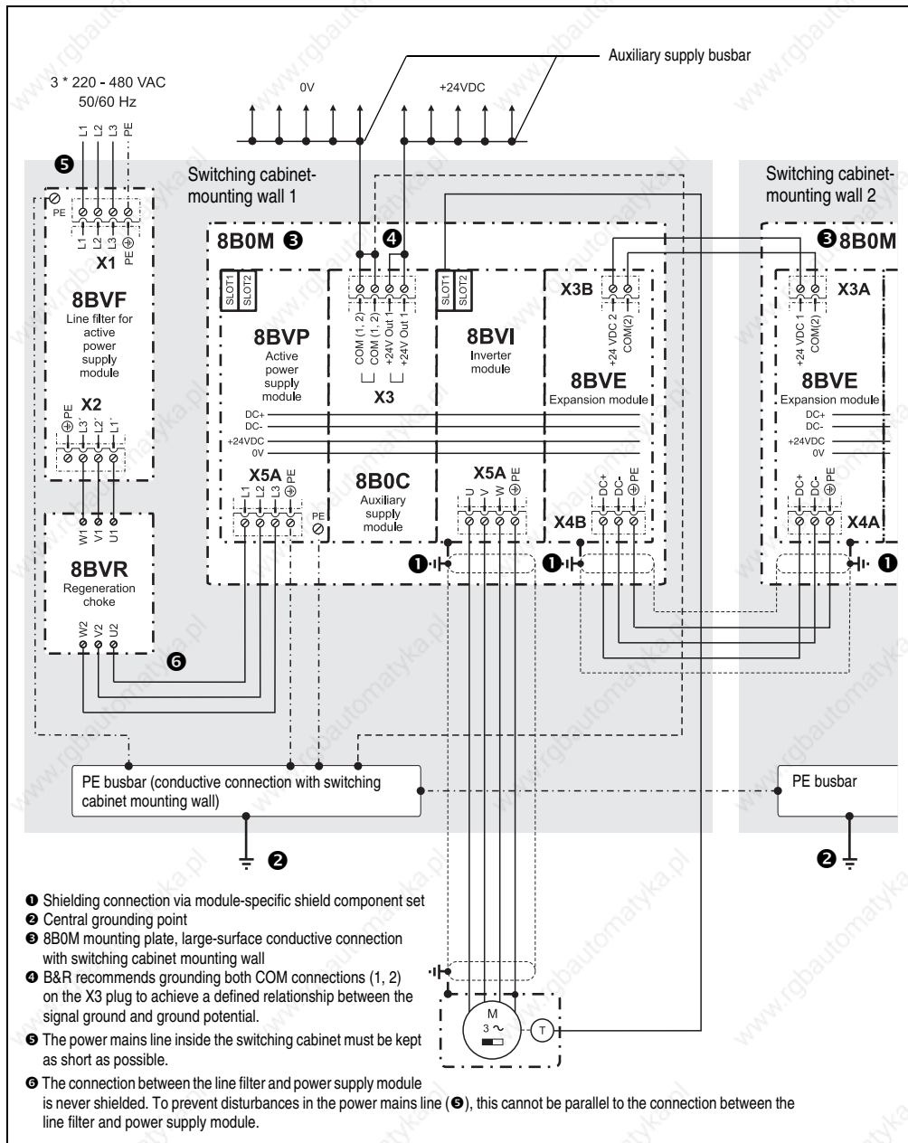
Figure 101: Overview of ground/shield for ACOPOSmulti drive system (active power supply)
