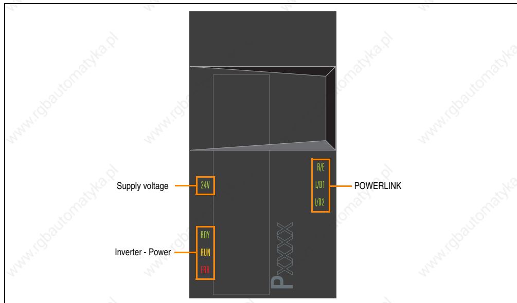
Figure 2: Indicator groups for 8B0P power supply units
