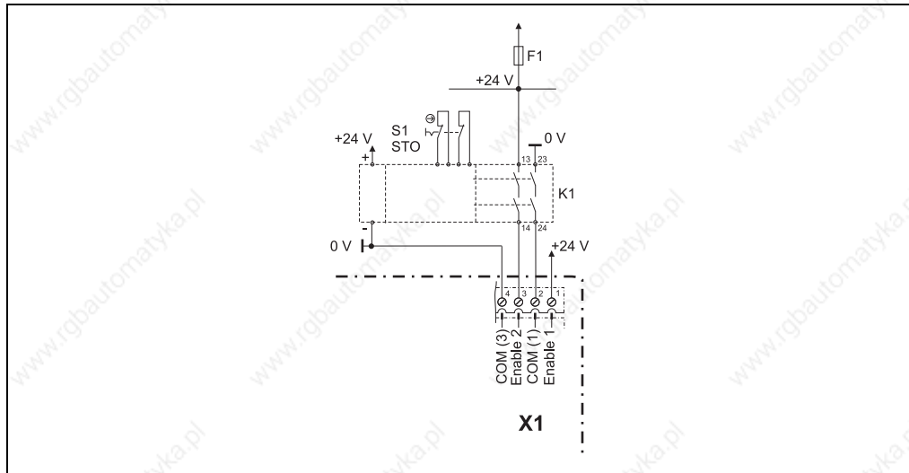
Figure 190: STO, Category 4 / SIL 3 / PL e (Variant A)
