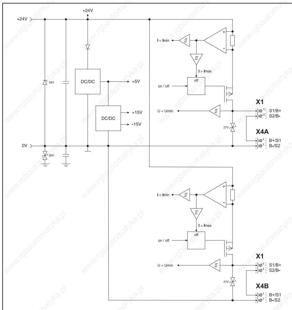
Figure 150: Input/output circuit diagram - 8BVI0014HxD0.000-1, 8BVI0028HxD0.000-1, 8BVI0055HxD0.000-1 (cont.)
