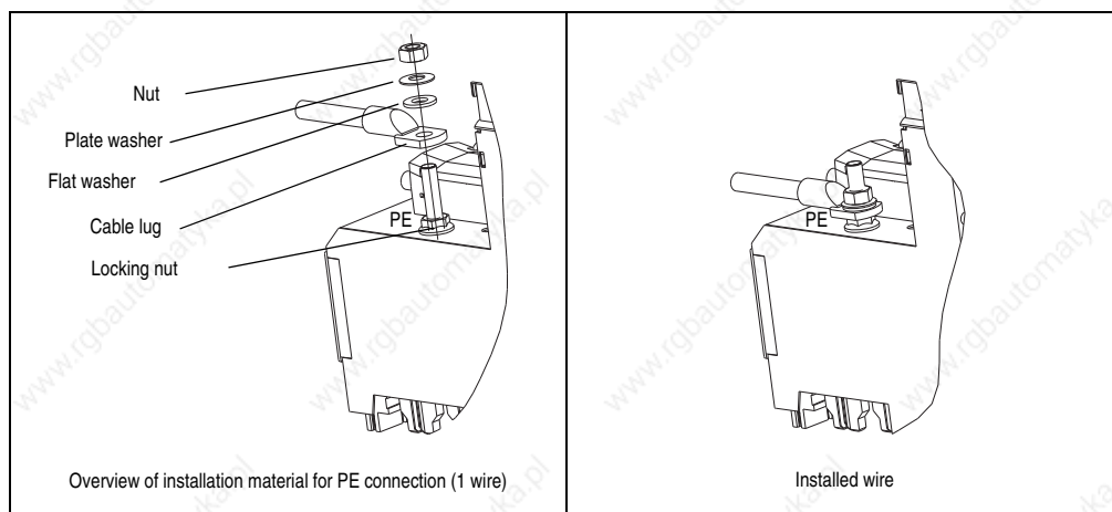
Figure 136: Cable installation connection PE (1 wire)
