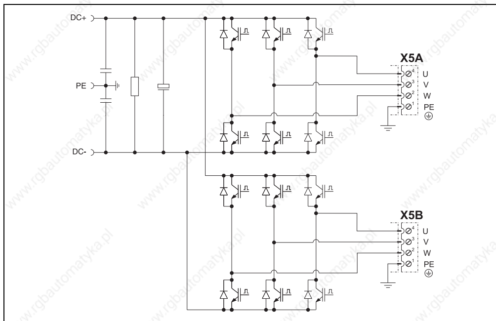
Figure 150: Input/output circuit diagram - 8BVI0014HxD0.000-1, 8BVI0028HxD0.000-1, 8BVI0055HxD0.000-1 (cont.)
