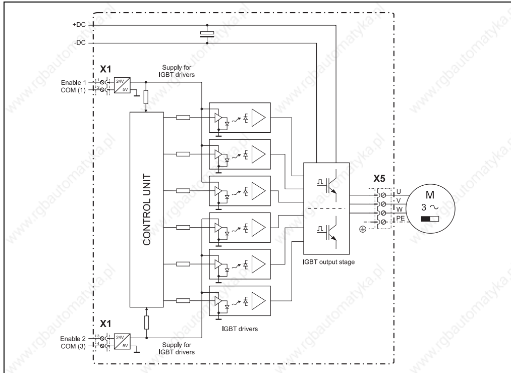
Figure 189: Block diagram of secure pulse disabling
