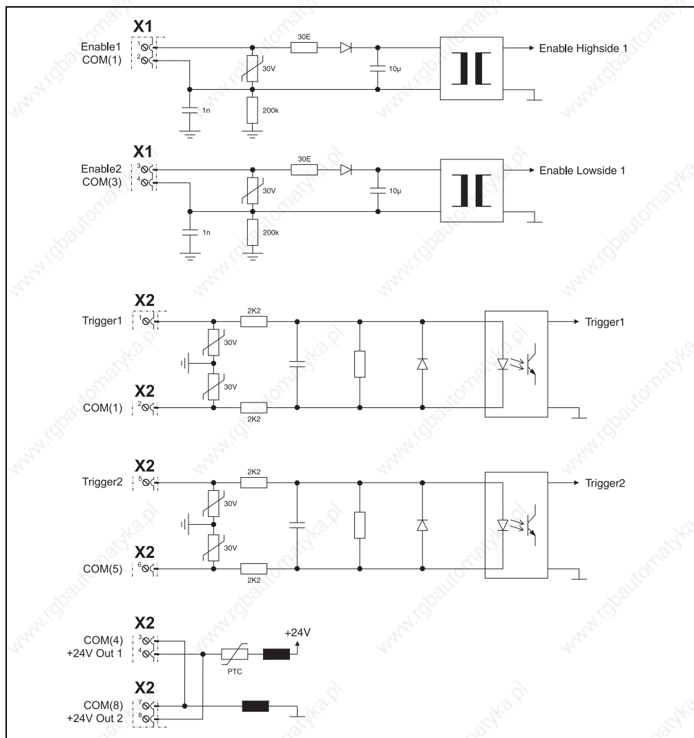
Figure 152: Input/output circuit diagram - 8BVI0220HxS0.000-1, 8BVI0440HxS0.000-1
