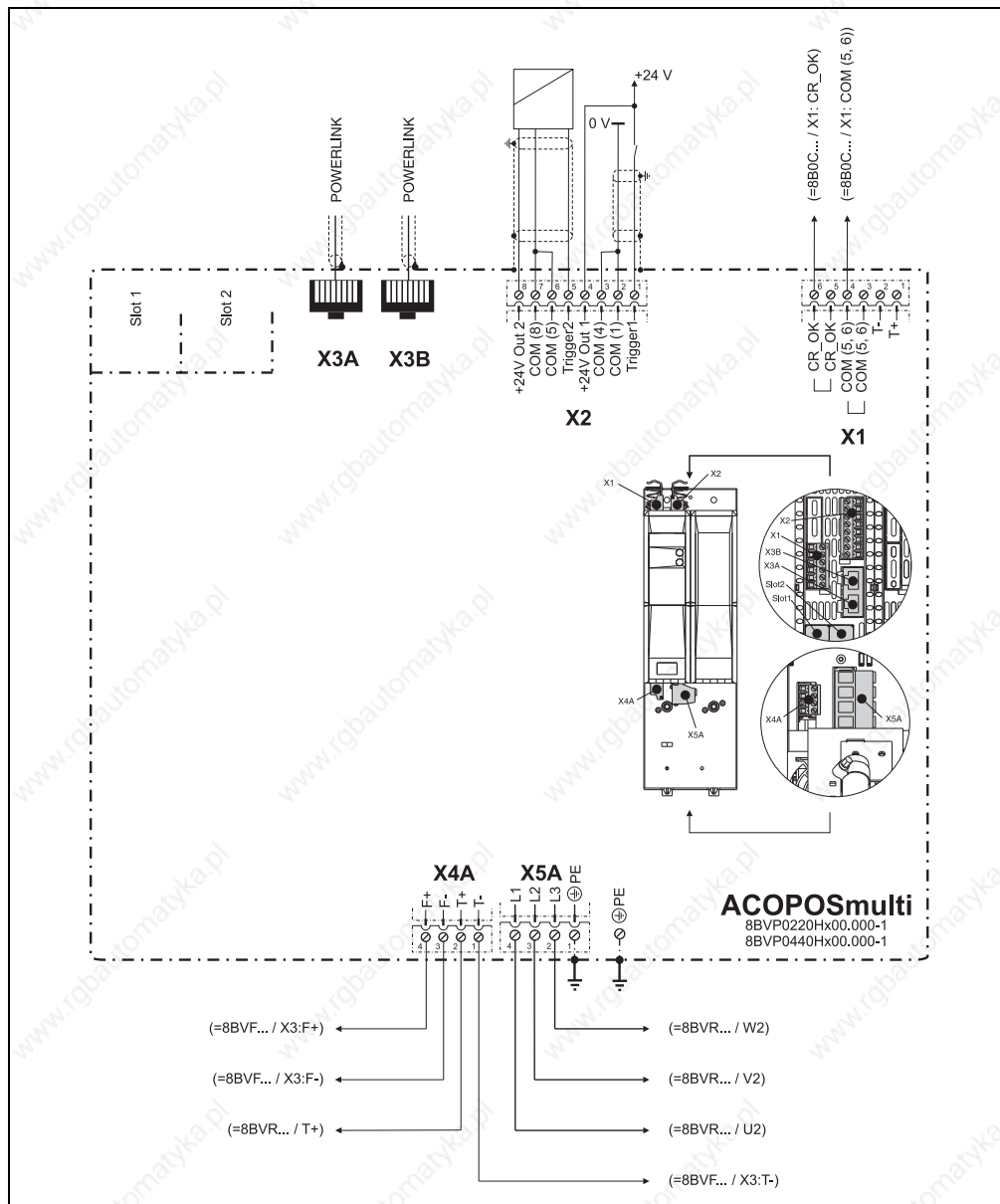
Figure 127: Overview of pin assignments - 8BVP0220Hx00.000-1, 8BVP0440Hx00.000-1
