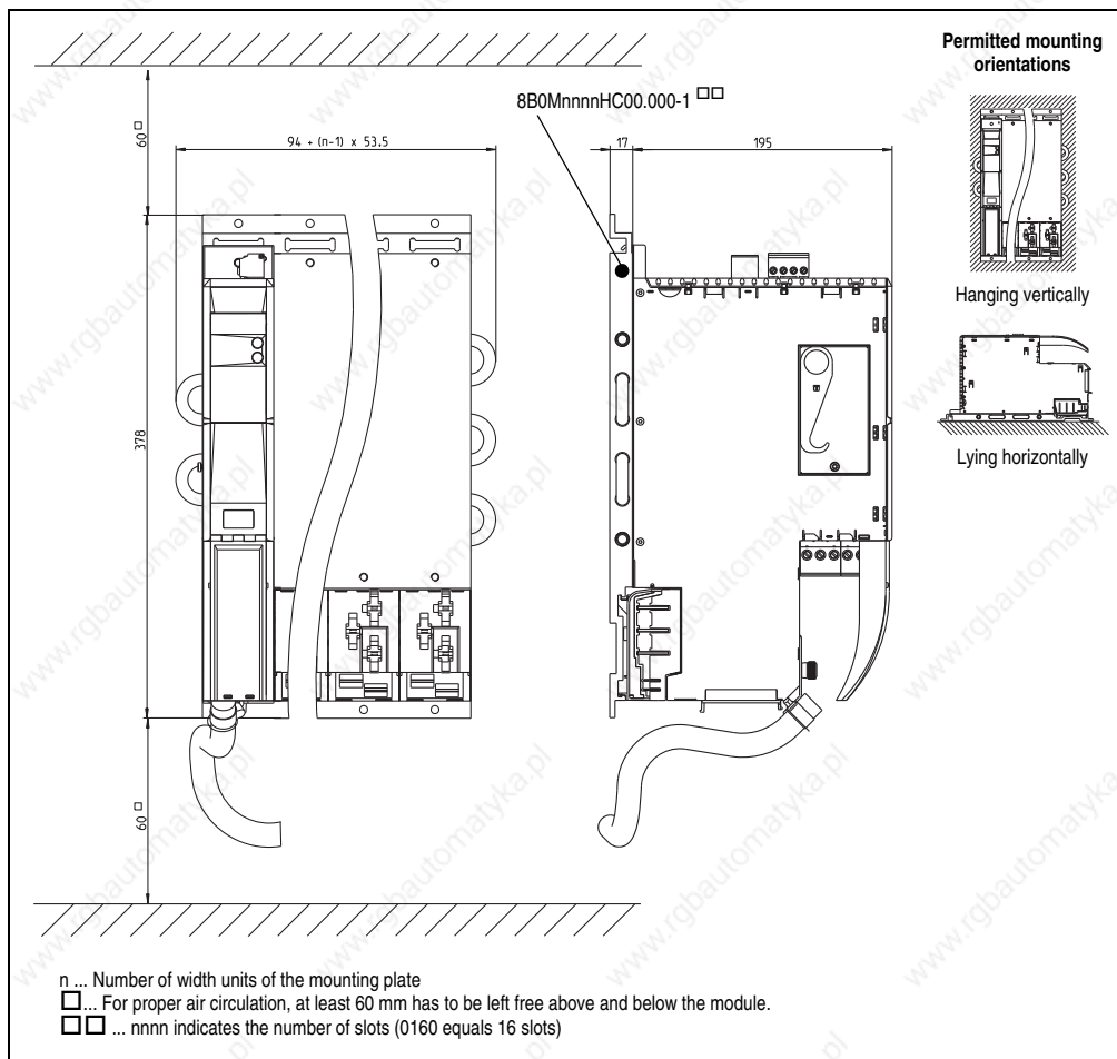
Figure 62: Dimension diagram and installation dimensions for 8BVE0500HC00.000-1
