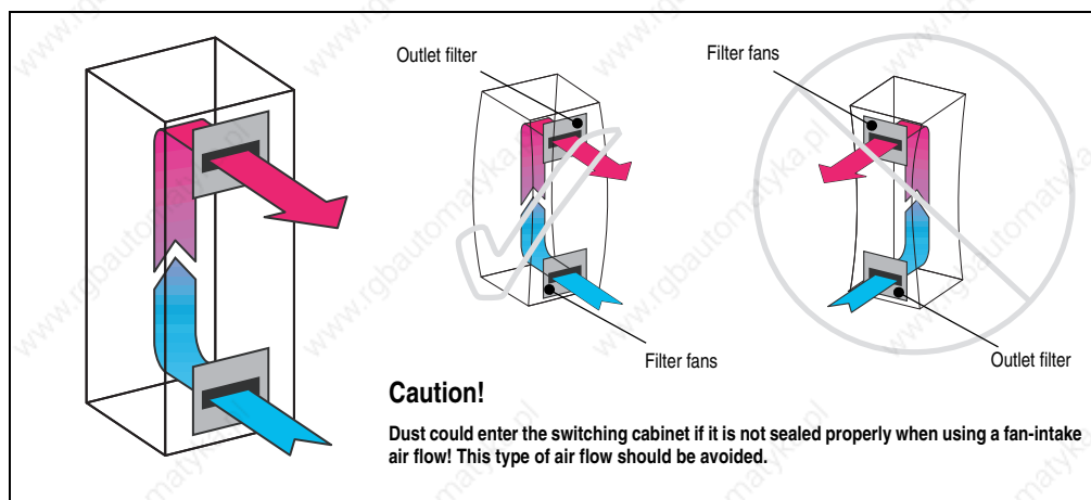
Figure 81: Function diagram of filter fans
