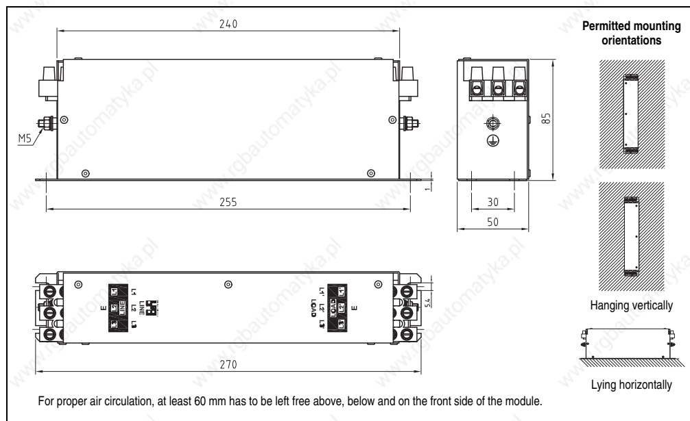
Figure 31: Dimension diagram and installation dimensions for 8B0F0300H000.000-1
