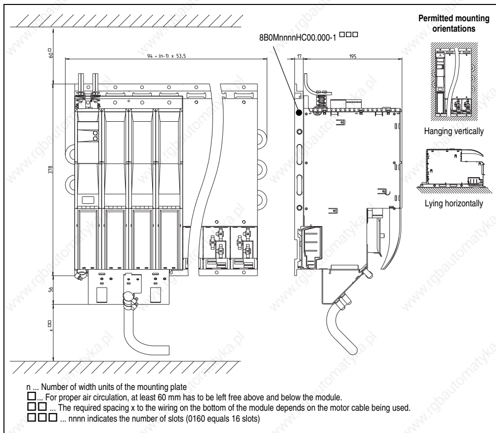
Figure 60: Dimension diagram and installation dimensions for 8BVI0880HCSx.000-1
