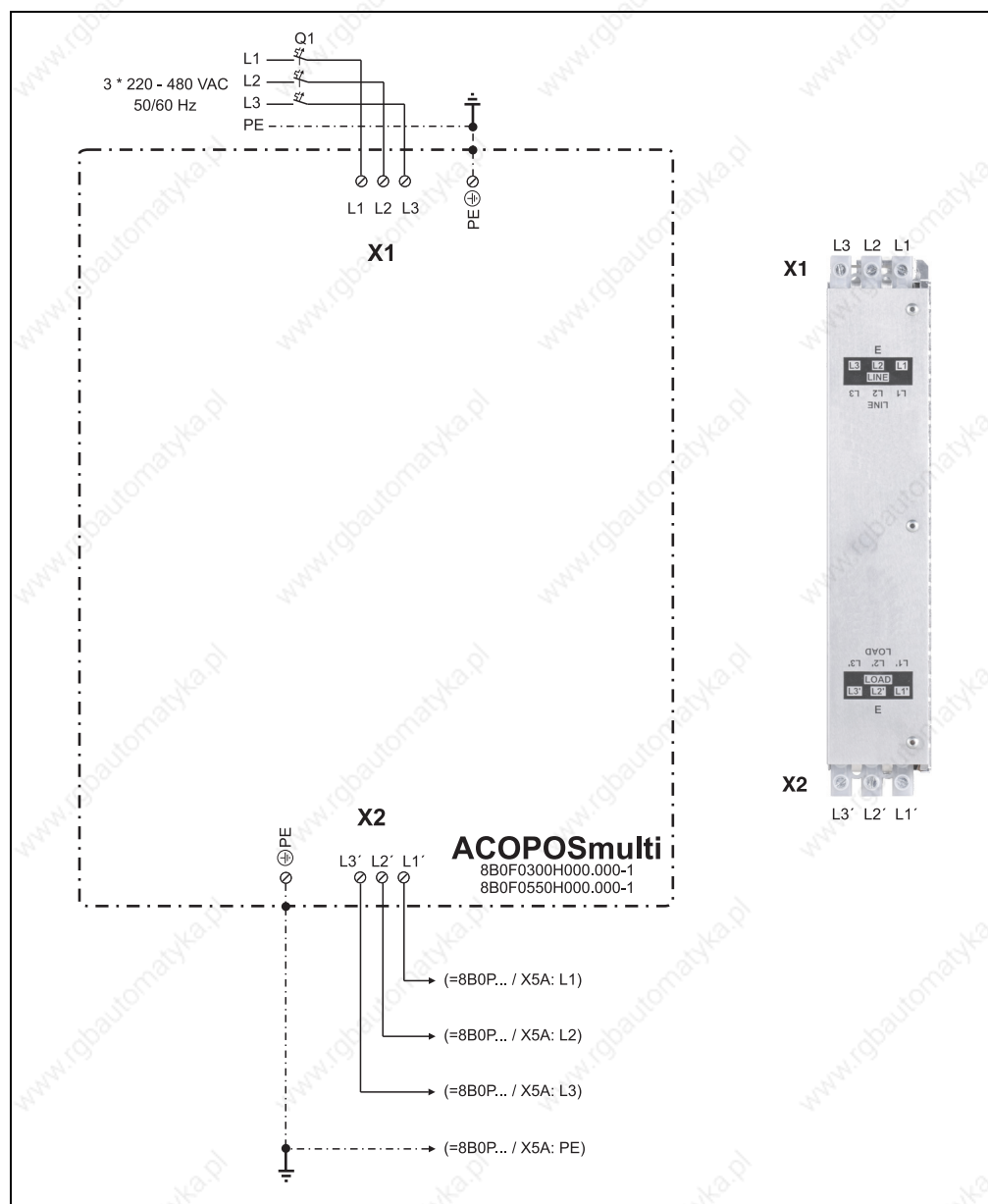
Figure 113: Overview of pin assignments - 8B0F0330H000.000-1, 8B0F0550H000.000-1
