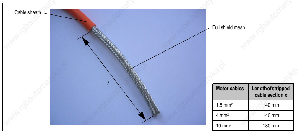
Figure 19: Stripped cable end
