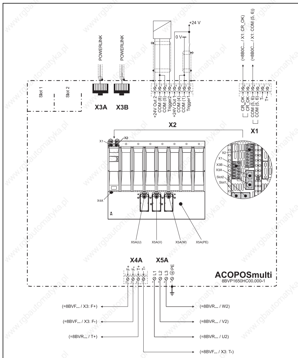
Figure 134: Overview of pin assignments - 8BVP1650HC00.000-1
