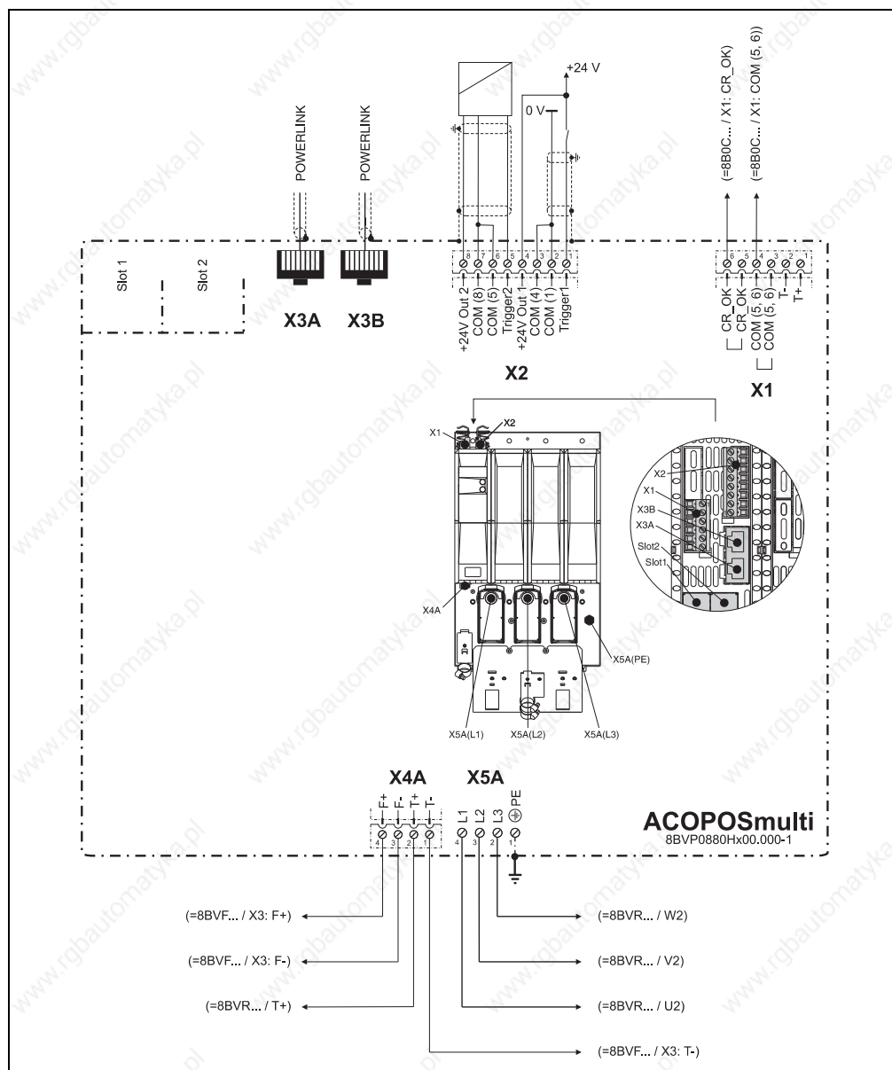
Figure 129: Overview of pin assignments - 8BVP0880Hx00.000-1
