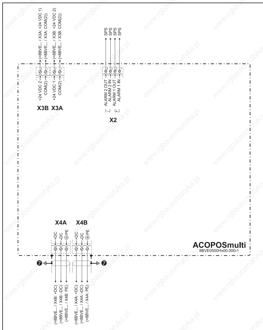
Figure 109: Ground connections and shield connections for 8BVE expansion modules
