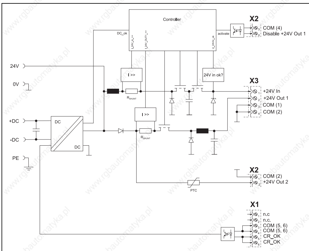
Figure 146: Input/output circuit diagram - 8B0C0320Hx00.00A-1
