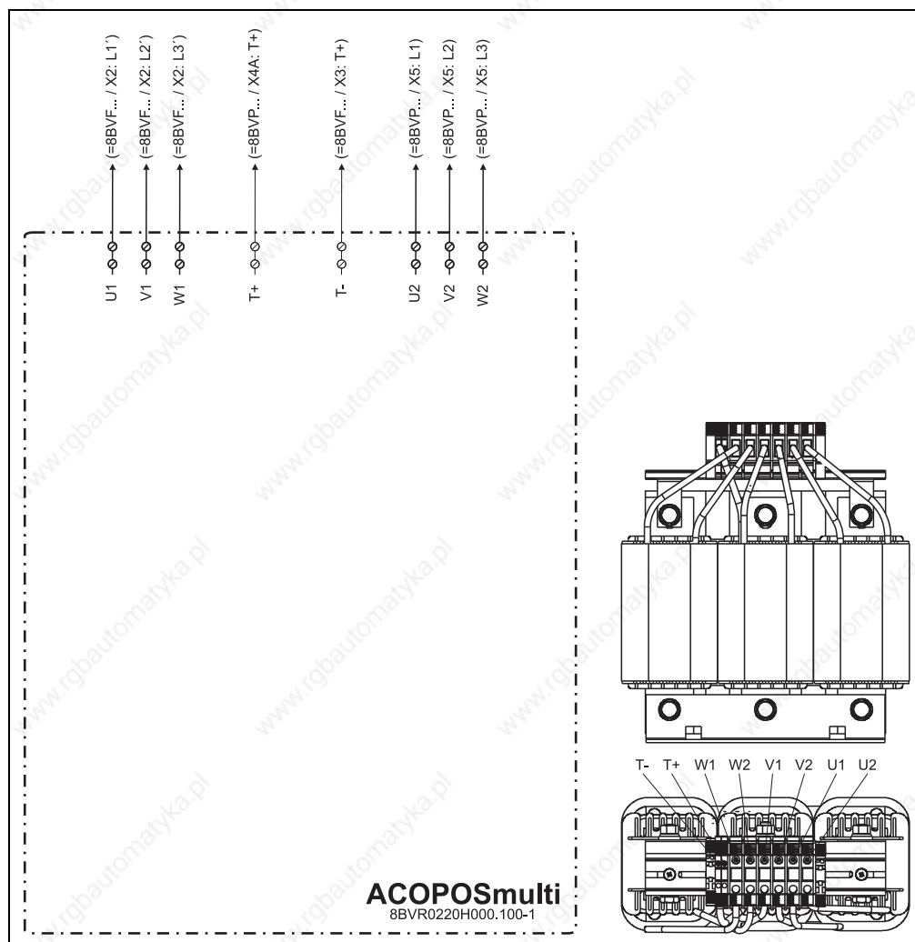
Figure 119: Overview of pin assignments - 8BVR0220H000.100-1
