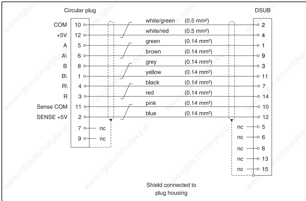
Figure 186: Cable schematic - 8BCS SinCos cable
